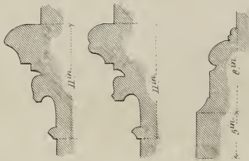
Section of Caps. & Base centre Pillars
