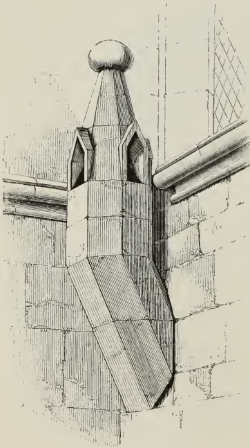
CHIMNEY OF THE LAVATORY, LINCOLN CATH.
