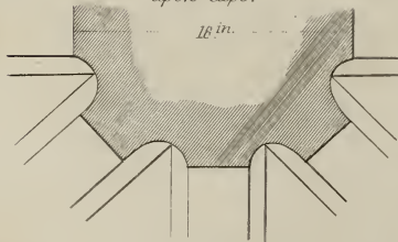
Plan of Groining upon Caps.
