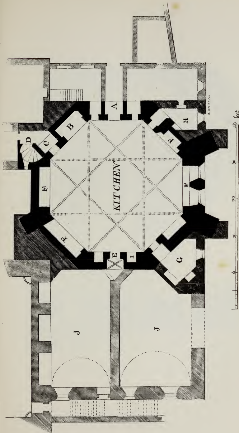
THE ABBOTS KITCHEN, DURHAM
