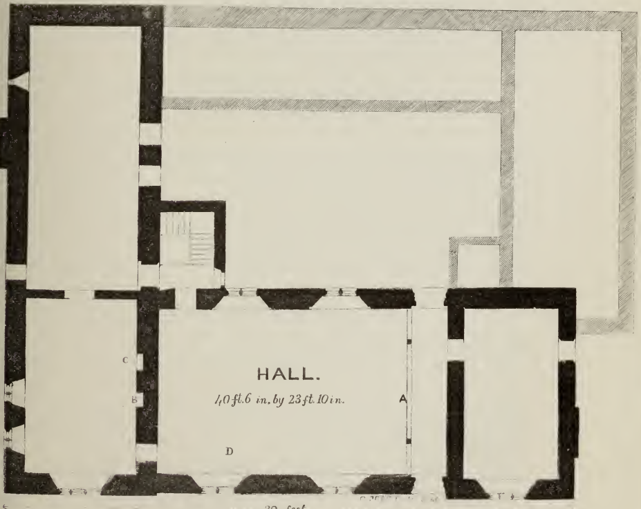
GROUND PLAN.
