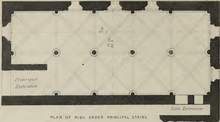
PLAN OF RIBS UNDER PRINCIPAL STAIRS
