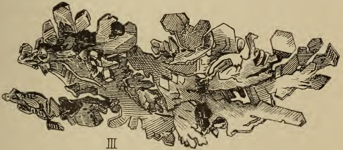
PSEUDOMORPHOUS GOLD.
