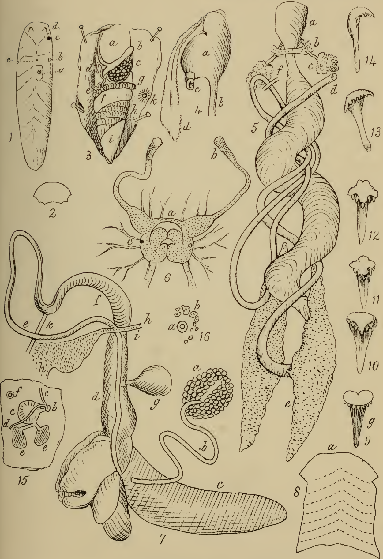
BITENTACULATE SLUG.
