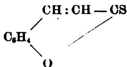
Thiocumarine.
