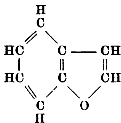
Cumarone.
