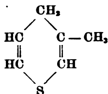
\beta -methylpenthiophene.
