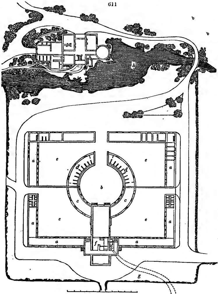
4173. An anomalous design for a corn and stall-feeding farm (fig. 611.), in which the stacks are built on the tops of the stables, cattle, and cart-sheds (a), may be noticed, as
