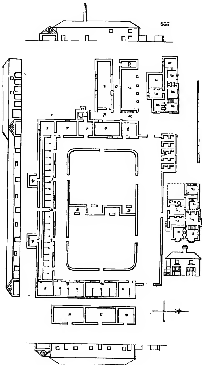
4163. As an example of a farmery to be managed by a bailiff, we give that of Skelho, also in Sutherland. The farm consists of 450 acres, the greater part taken from a heathery waste. It contains a suitable house for the grieve or bailiff, and attached to the office is a threshing machine, combining a corn or meal-mill. Its accommodations
