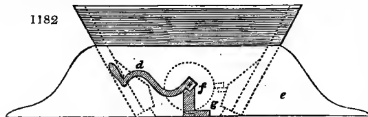
in length, and is moved by the crank handle (d in fig. 1182.); c e are two wedge-shaped pieces of hard wood,
