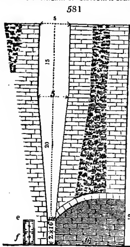
3864. Menteath or Closeburn coal lime-kiln. When lime is to be burned with coal or smoky fuel, a form
