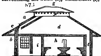
7006. The fixtures of the dairy are, in the scalding-room, a copper boiler fixed over a
