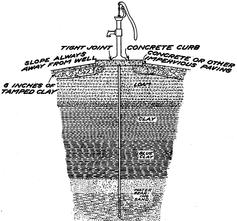
FIG. 20.—Driven well.
