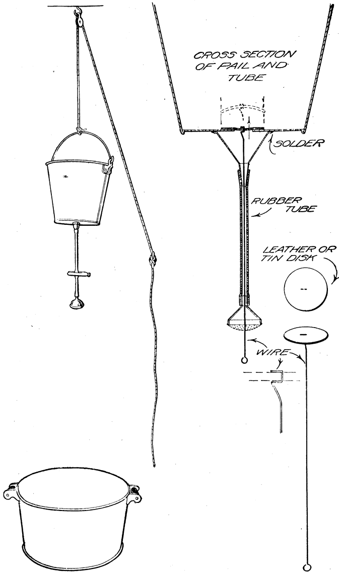
FIG. 16.—The shower bath.
