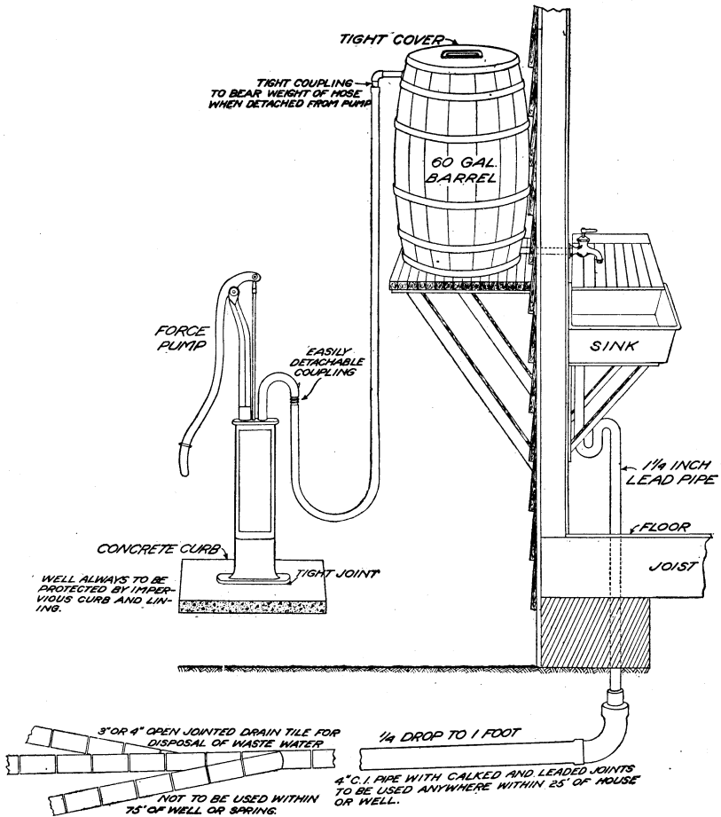
FIG. 21.—Simple water-supply system for farm kitchen.
