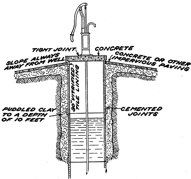
Fig. 18.—Dug well, vitrified tile lining.
