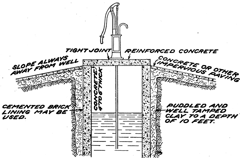
Fig. 17.—Dug well, concrete or cemented-brick lining.
