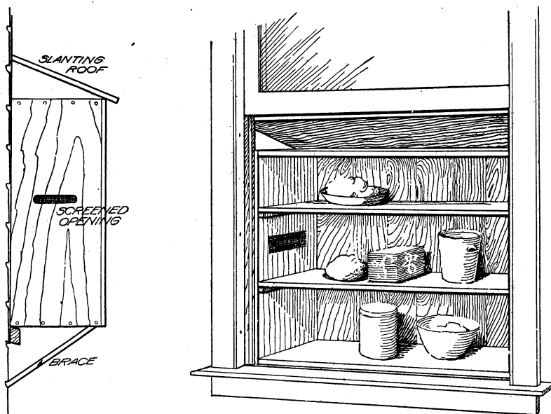
FIG. 13.—Cold box.
