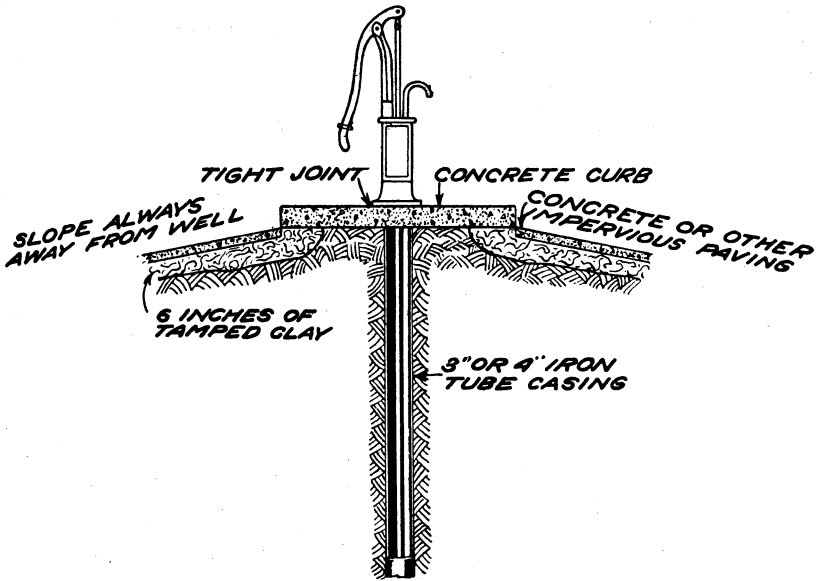
FIG. 19.—Bored well.
