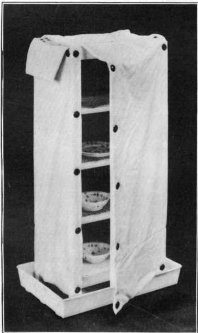
FIG. 12.—The completed iceless refrigerator.
