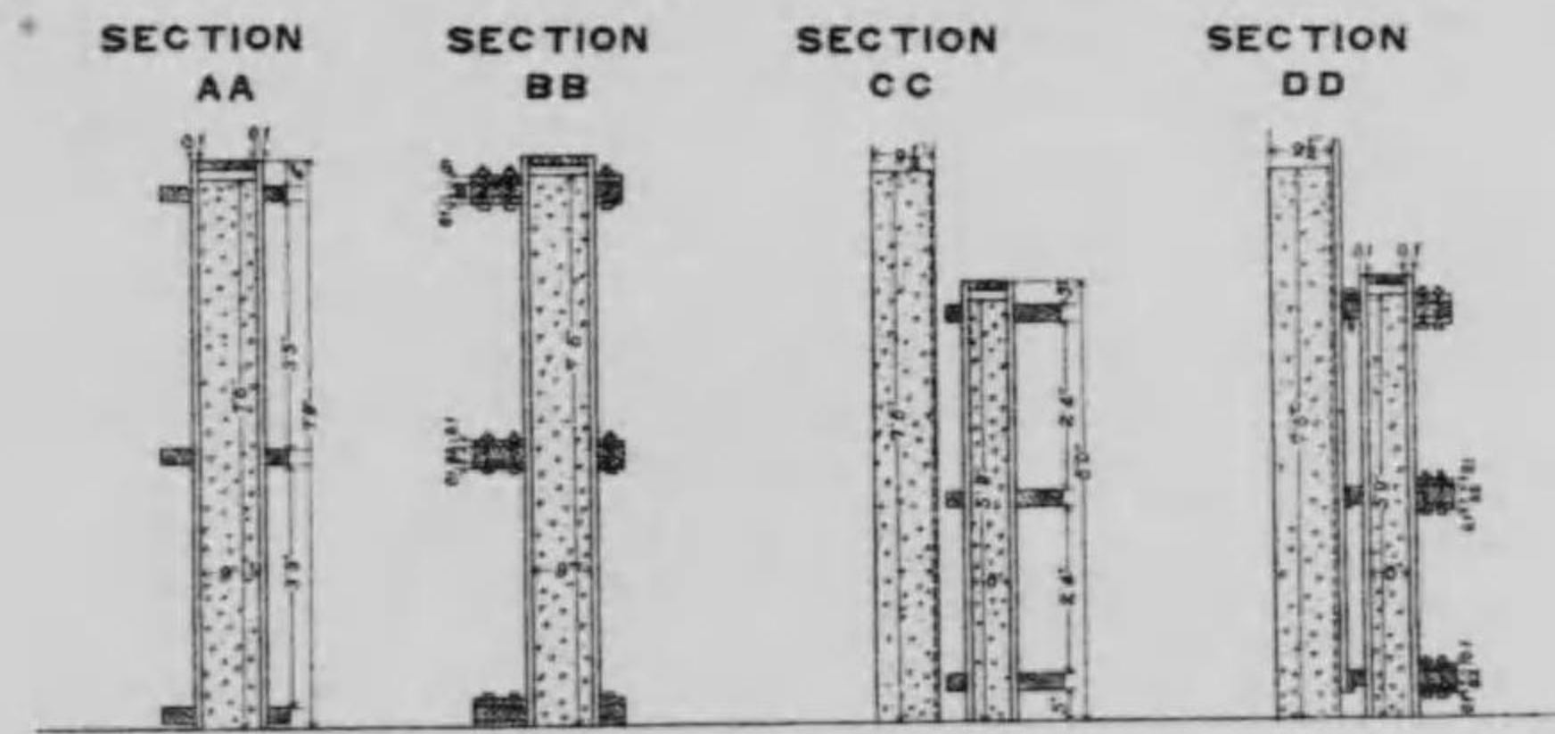
SECTIONAL ELEVATION
