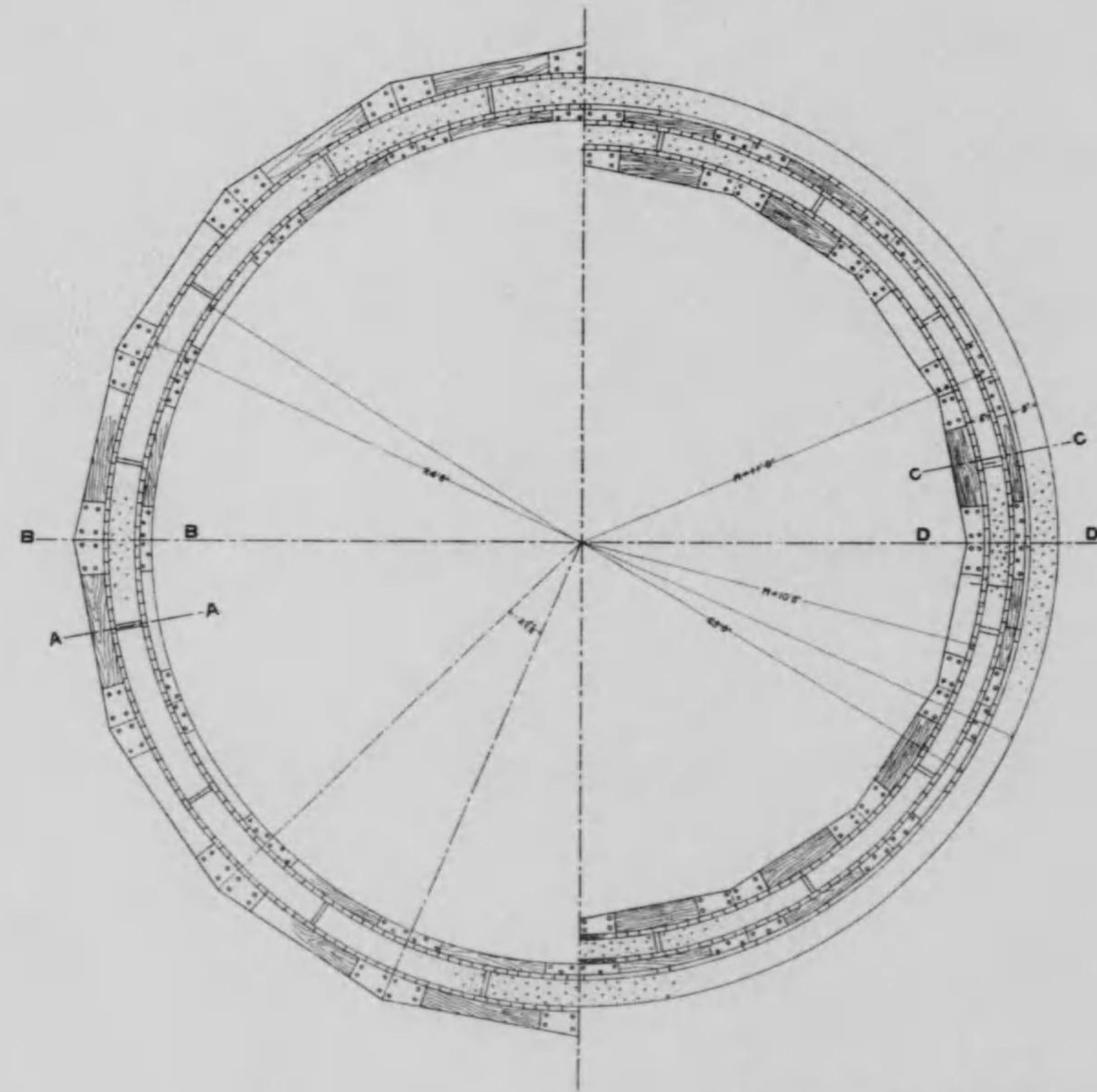
SECTIONAL PLAN
