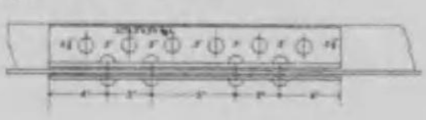
JOINT OF CHORD
