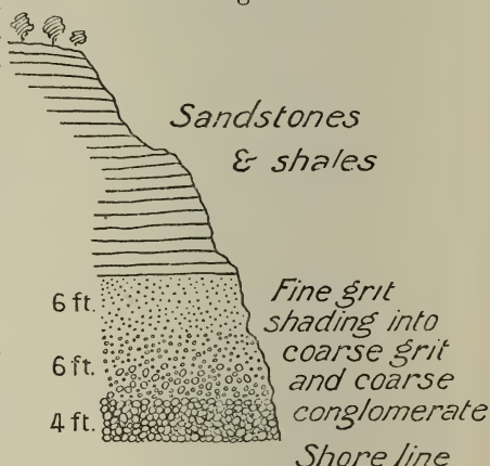
Section at end of point, Whangaparaoa.
