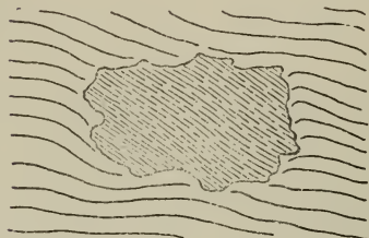
Included block of andesite, 18 ft. across, imbedded in sandstone and shale at Whangaparaoa.
