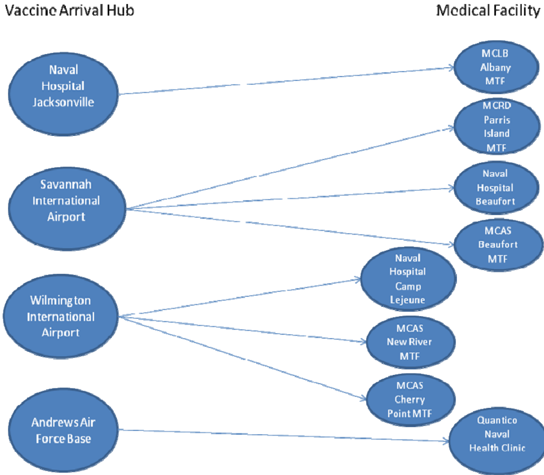
Figure 11. Transportation Model
