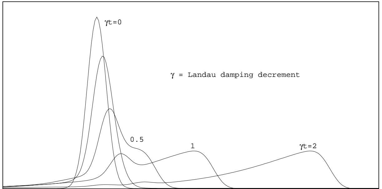
Wave energy carried away by resonant electrons
