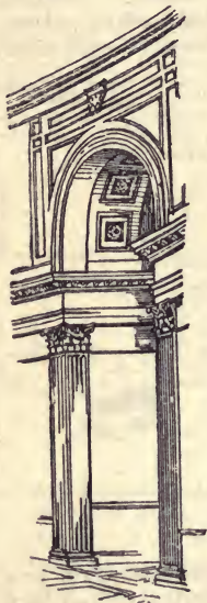
Section of Pantheon
