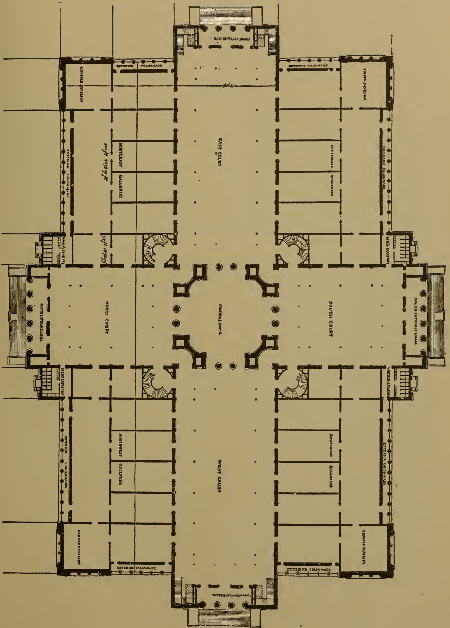
FLOOR PLAN OF THE FINE ARTS.—WORLD'S COLUMBIAN EXPOSITION.
