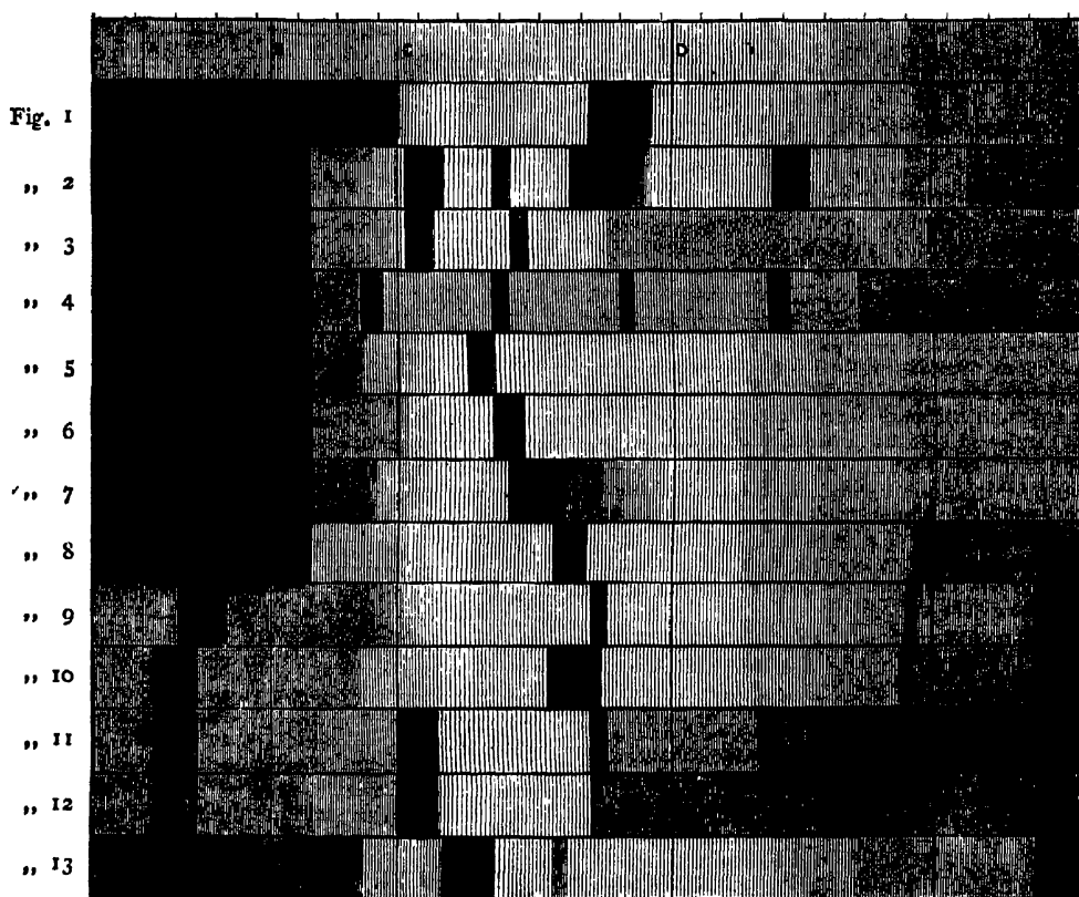
1, Water; 2, Ammonia; 3, Ammonia in Alcohol; 4, Ethylamine; 5, Amyl Alcohol; 6, Ethyl Alcohol; 7, Aldehyde; 8, Acetic Acid; 9, Benzene; 10, Toluene; 11, Aniline; 12, Toluidine; 13, Turpentine.
