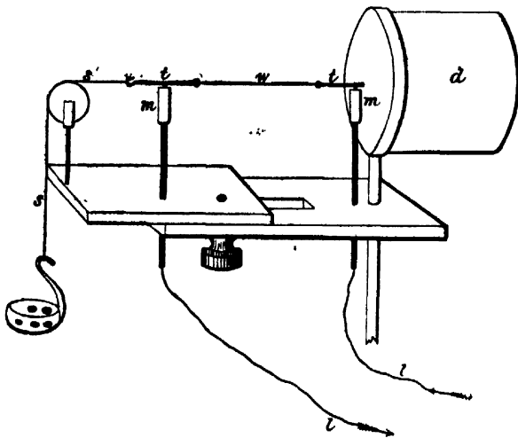
w , fine wire; t t , thicker copper terminals; m m , mercury cups over which t t pass; s s , string kept tight by small load; l l , line wires to microphone; d , drum head which distributes the sound.
