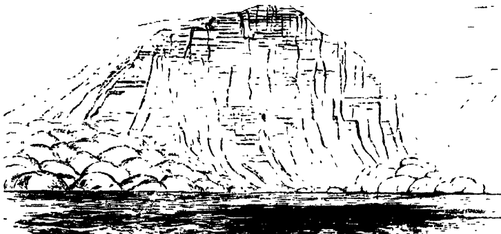
FIG. 2.—Ben Shieldag, Loch Torridon—a hill of flat Cambrian red sandstone resting upon an uneven hummocky surface of the old gneiss.
