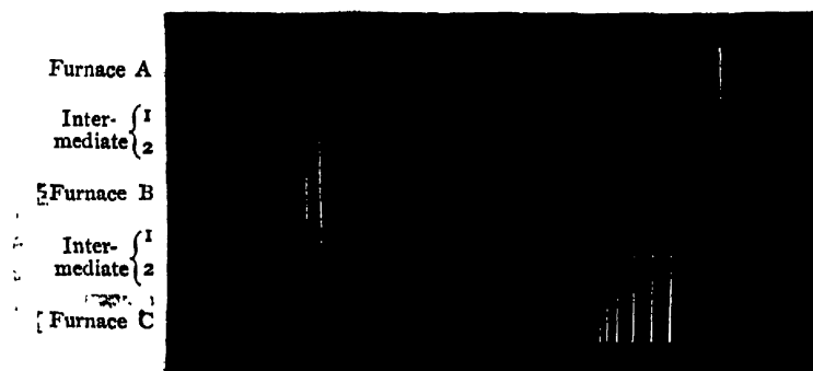
FIG. 4.—Spectra of the hypothetical substance in intermediate furnaces, assuming that the vapours are not completely dissociated.
