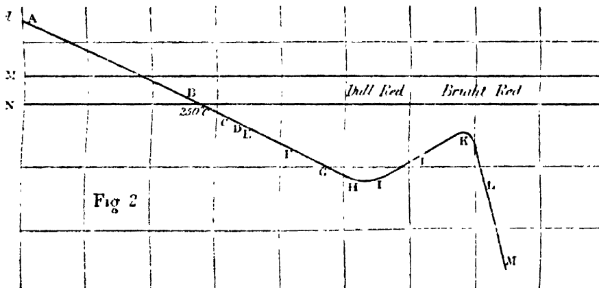
FIG. 2.—Steel.—A, sizzling sound and high note, neither loud; B, silence; C, high note comes in again; D, sharp sizz; E, buzzing sound and general increase of loudness. The other letters as with iron.
