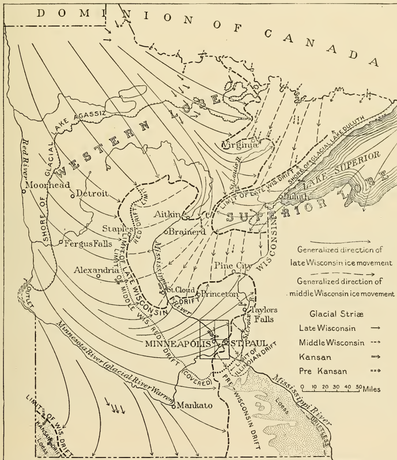
FIG. 25. Map of Minnesota Showing the Extent of the Glacial Ice Sheets, Direction of Ice Movements, and Shores of Glacial Lakes. By Frank Leverett.
