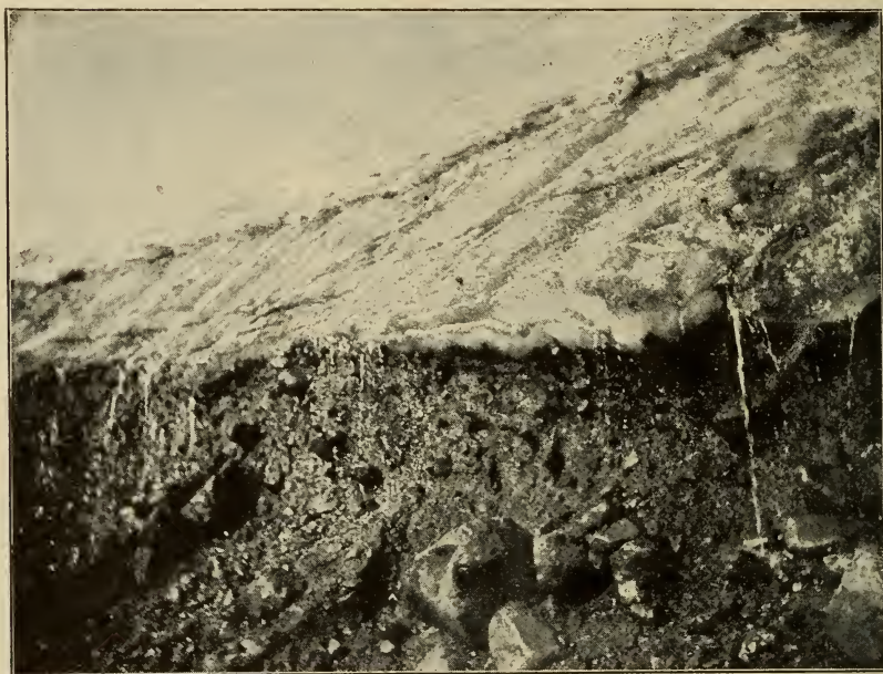
FIG. 11. Showing Moraine which is being Crowded upon by the Moving Ice. Photograph by Prof. T. C. Chamberlin.
