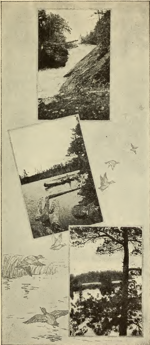
Fig. 45a. Superior National Forest, Ely. Falls of Isabella River; Kawishwi River; Gabro Lake.
