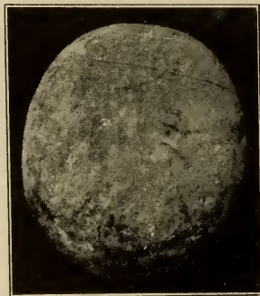
FIG. 96. A Grinder from a Pot Hole, The Dalles of the St. Croix, Taylor's Falls. Photograph by Brown.
