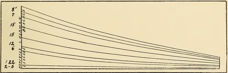
FIG. 81. Diagram Showing the Progressive Elevation of Beaches Northward in Vicinity of Maple Lake, Minn. Continue the Lines to the Right and the Upper Five Meet in One, and the Lower Four in One.
