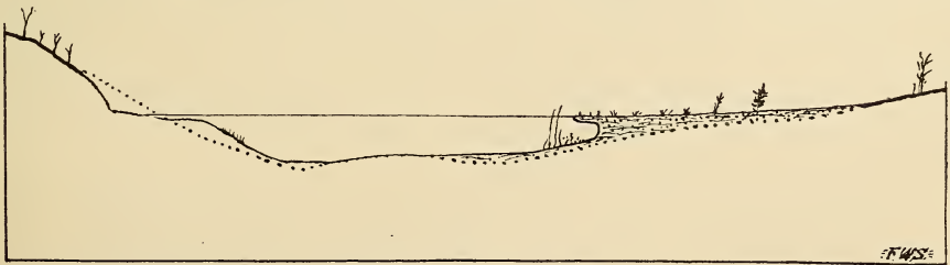
FIG. 56. Cross Section of a Lake Showing Wave-cut Shore (left) and Bog Filling (right).
