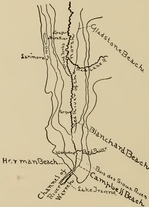
FIG. 74. During the Higher Stages the Lake Outflowed Southward. The Lower Beaches Cross the Red River of the North.
