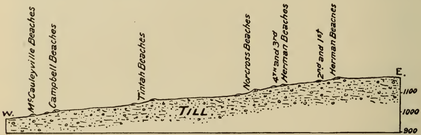
FIG. 79. Profile of Beaches. West of Maple Lake.
