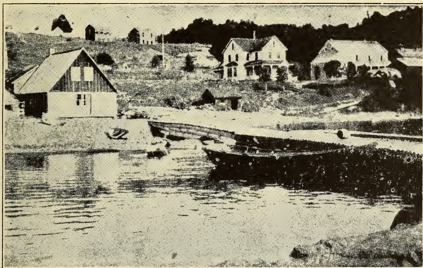
FIG. 103. Terraces Showing the Higher Levels of Lake Duluth at Lutzen, Cook County.
