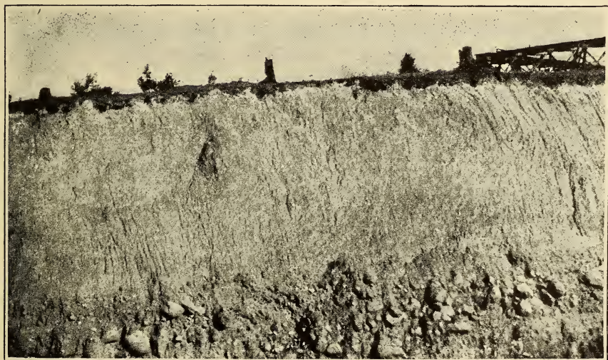
FIG. 30. Clayey Keewatin Drift over Stony Patrician Drift at Biwabik. Photograph by F. J. Alway.
