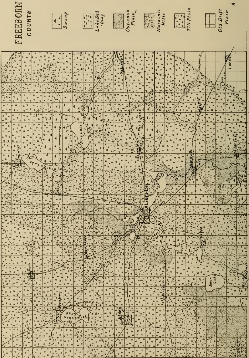
FIG. 106. Map Showing Details of Glacial History in Freeborn County. Drawn by F. W. Sardeson.
