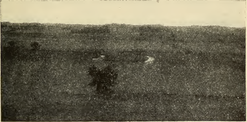
FIG. 43. An Old Valley in Driftless Area of Minnesota.
