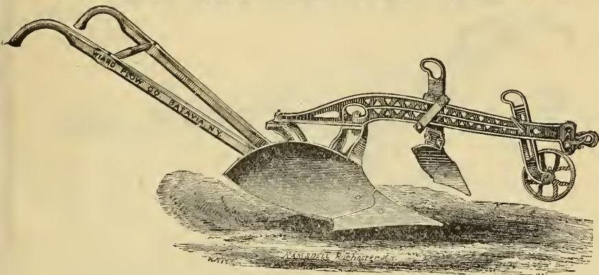
WIARD'S PATENT ADJUSTABLE MALLEABLE IRON BEAM CHILLED PLOW. Centre Draft. Right Hand.
