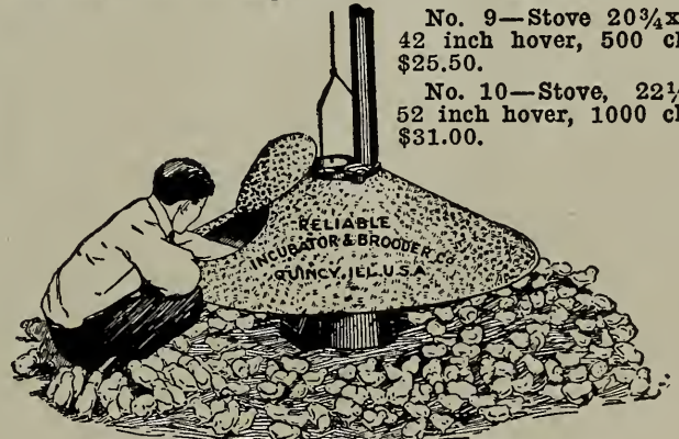
New Reliable Coal Burning Brooder.
