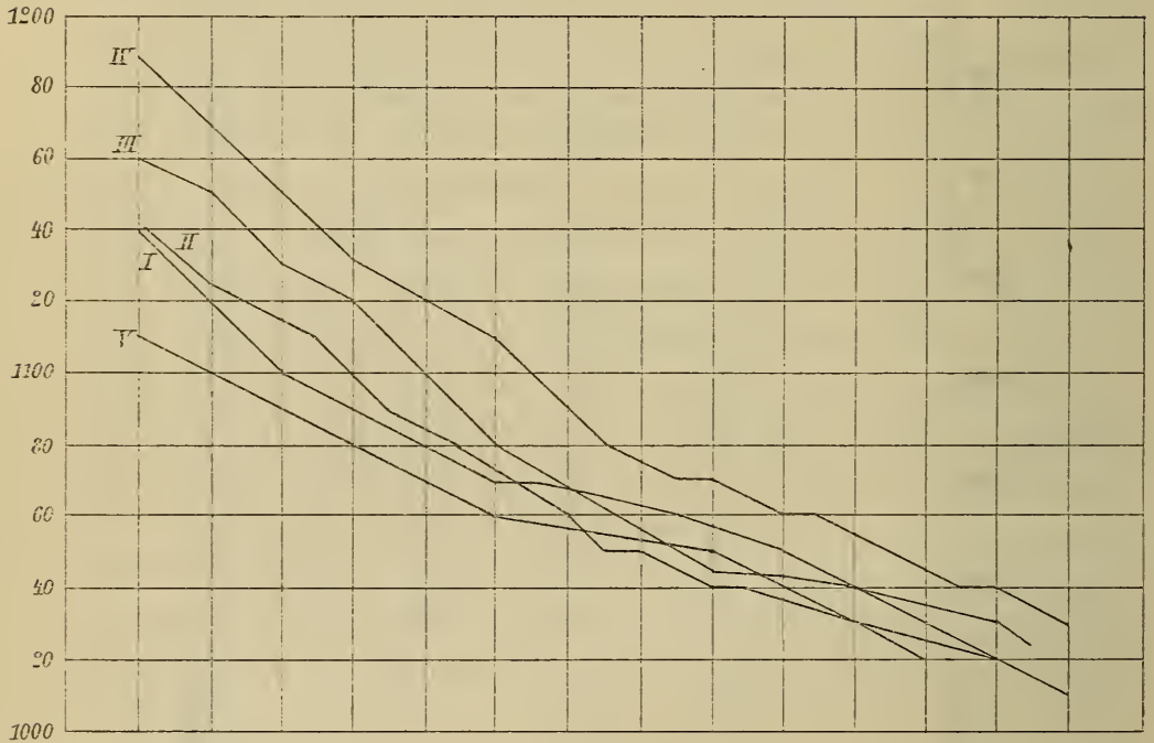
Fig. 8. Labrador-Nephelin (Mineralgemenge).
