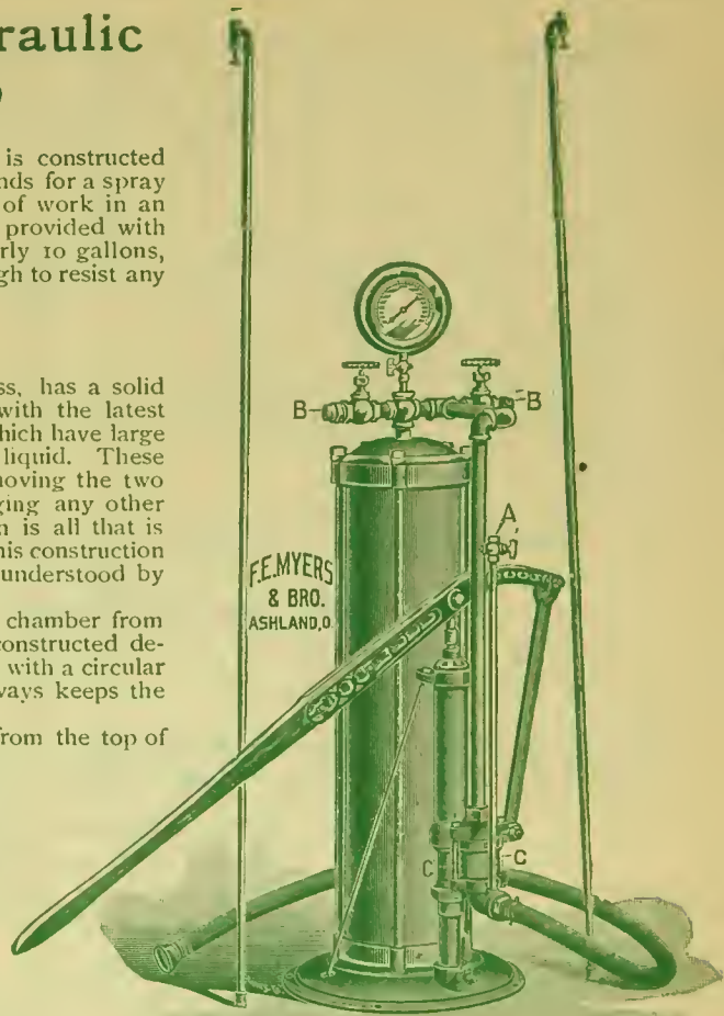
HYDRAULIC SPRAY PUMP.
