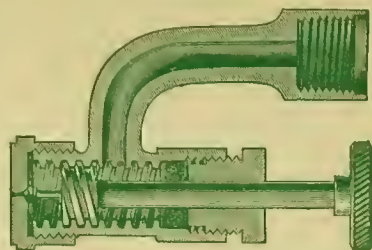
MYERS GRADUATING SPRAY NOZZLE
