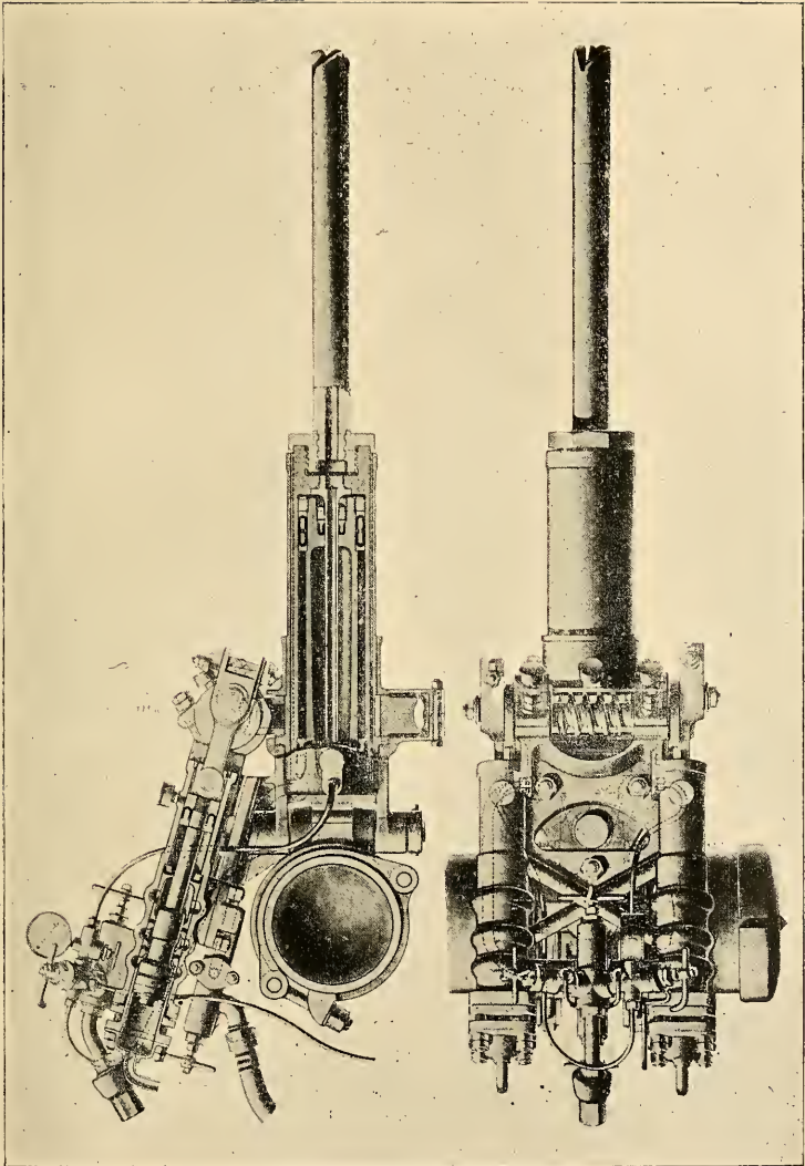
Tafel 4: Bohrmaschine.
