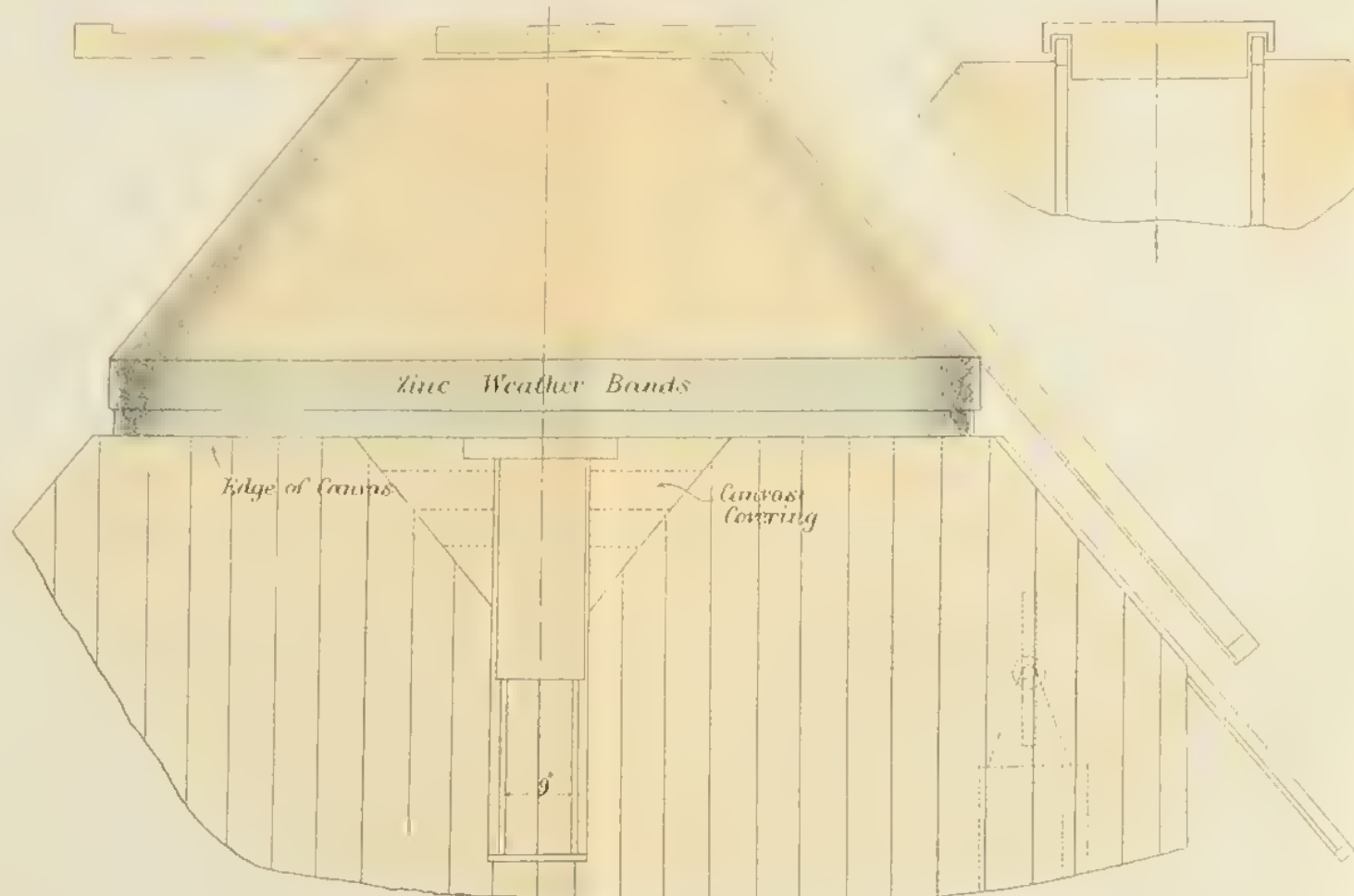
FRONT VIEW OF TRANSIT SHUTTER. SIDE VIEW OF SHUTTER SLIDES.
