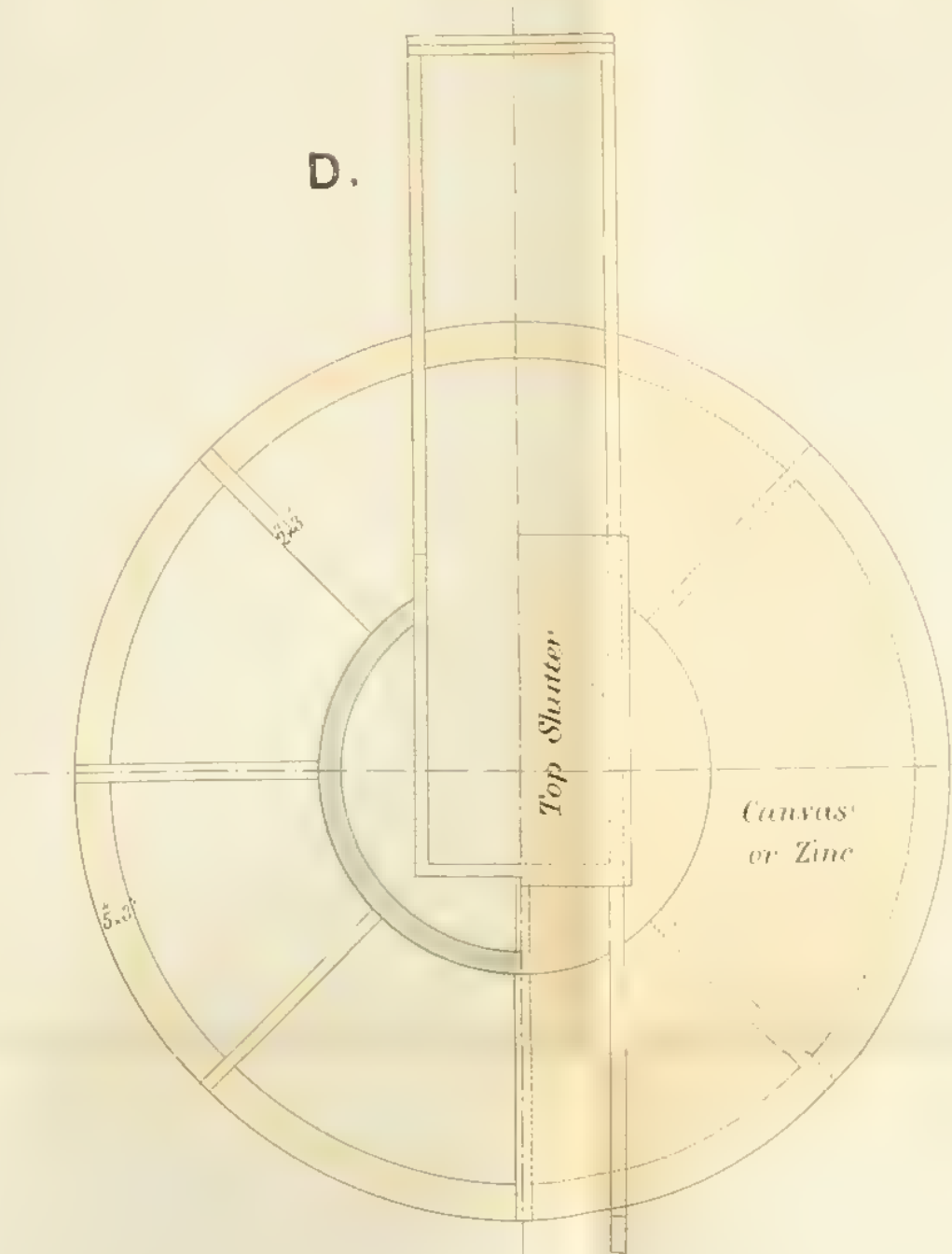
PLAN OF TOP OF DOME.
