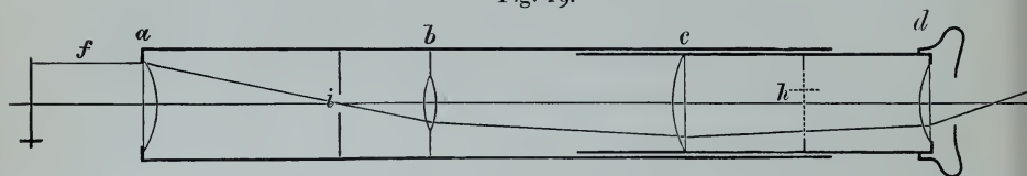
THE TERRESTRIAL EYE-PIECE.
