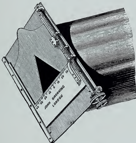
KNOBEL'S ASTROMETER.
