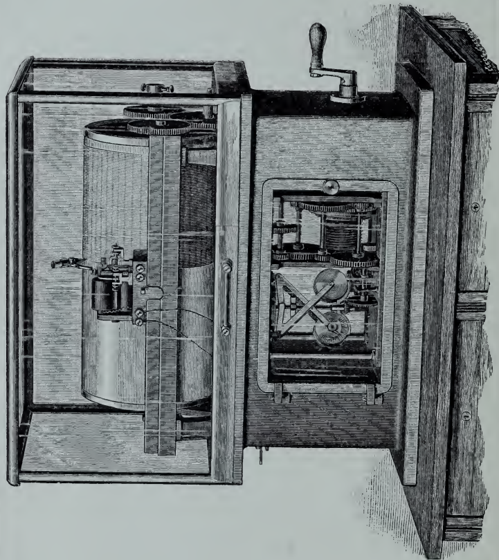
AMERICAN CHRONOGRAPH.
