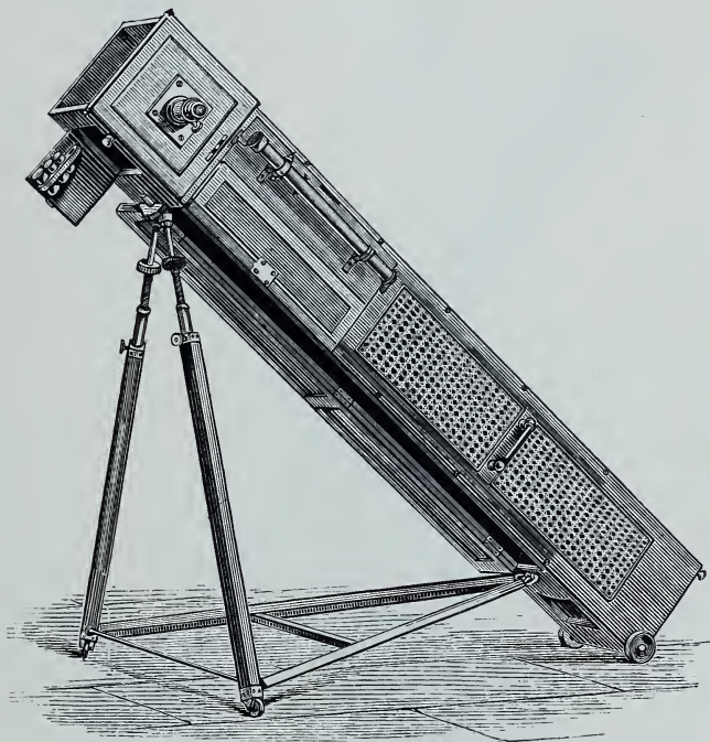
ALTAZIMUTH MOUNTING FOR REFLECTORS.
