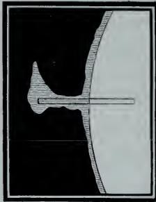
SLIT PLACED RADIALLY TO VIEW A PROMINENCE.
