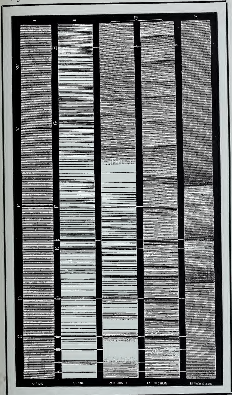
SECCHI'S TYPES OF STELLAR SPECTRA.
