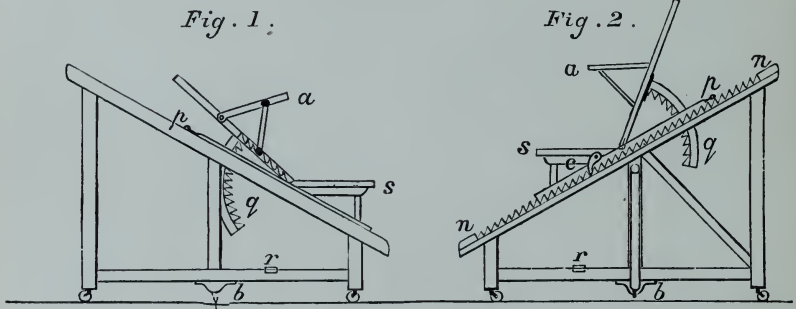
DAWES'S OBSERVING CHAIR.
