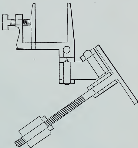
WINDOW EQUATORIAL MOUNTING. ( Erck. )
