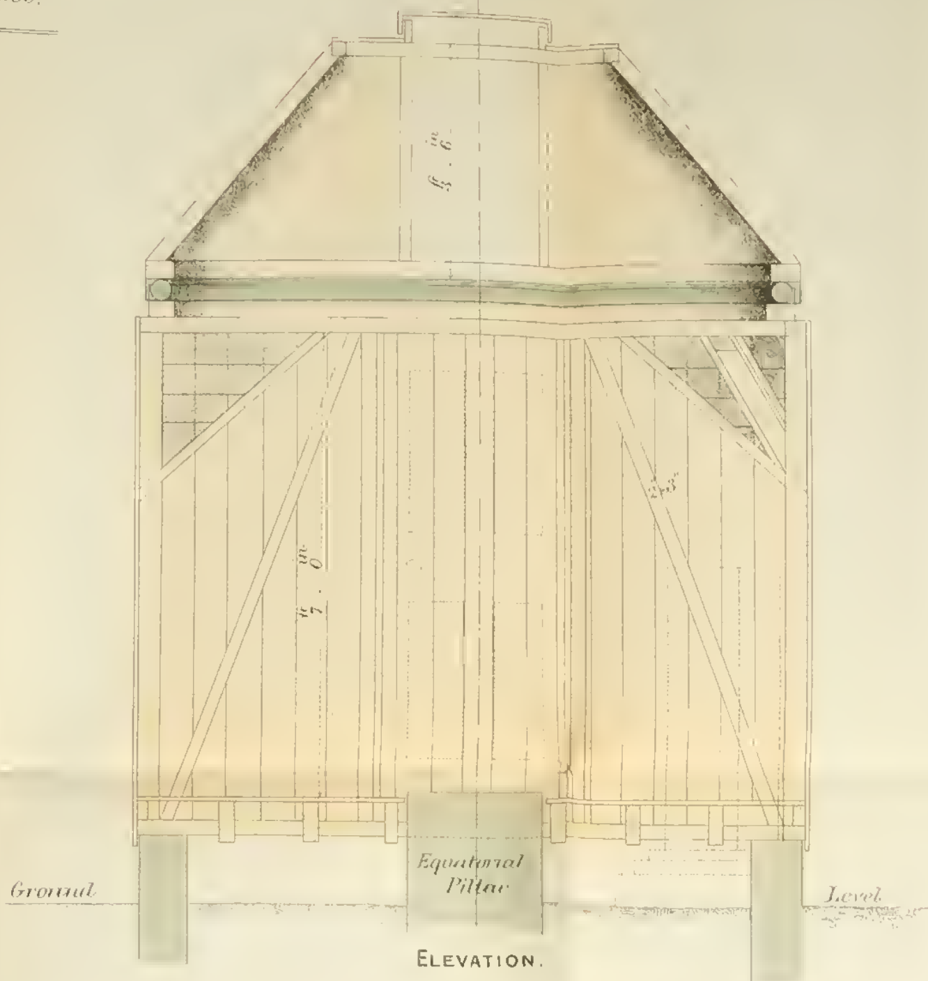
ELEVATION OF END OF TOP SHUTTER, Made to lap over Dome Shutter
