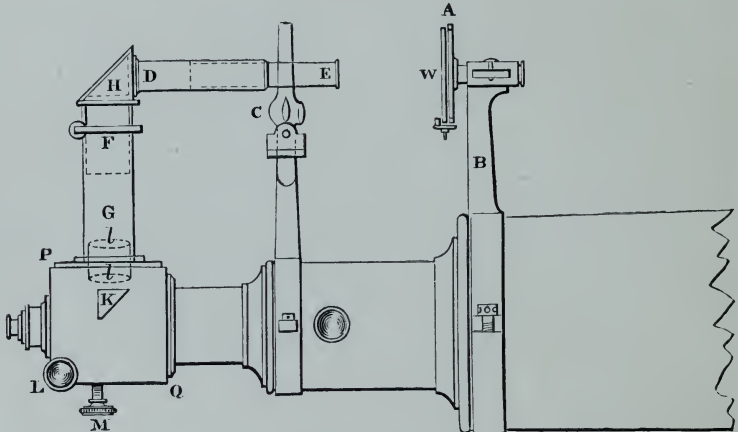
BIDDER'S MICROMETER.
