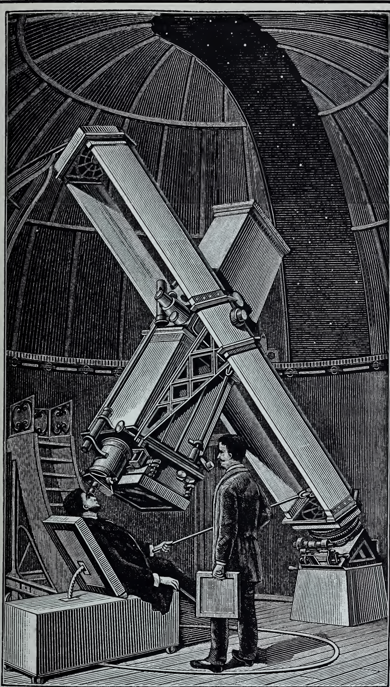
THE ASTRO-PHOTO-HELIOGRAPH OF THE PARIS OBSERVATORY.
