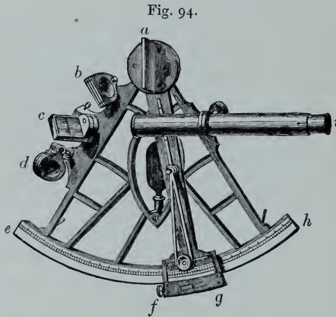
THE SEXTANT.
