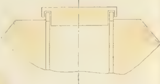
ELEVATION OF END OF TOP SHUTTER, Made to lap over Dome Shutter
