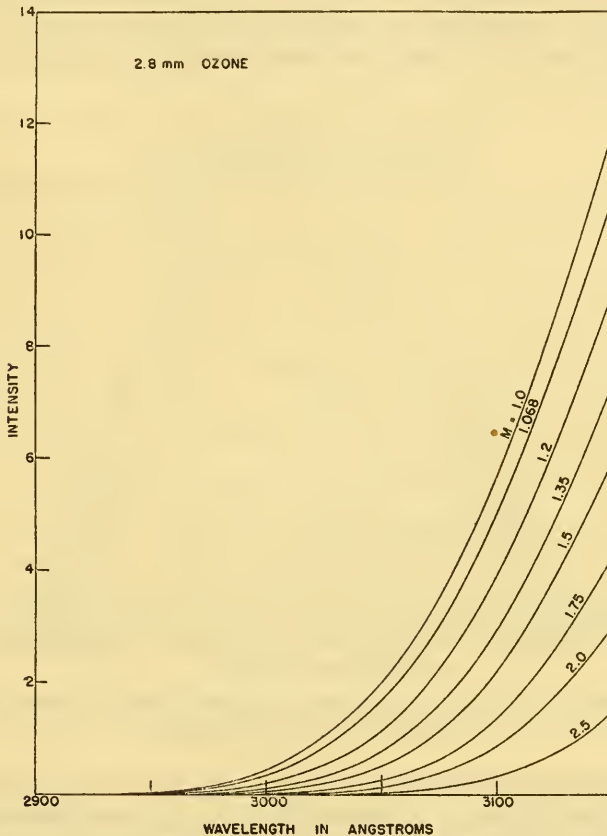
FIGURE 8.—Solar spectral energy for various air masses. (2.8 mm. ozone in zenith atmosphere.)
