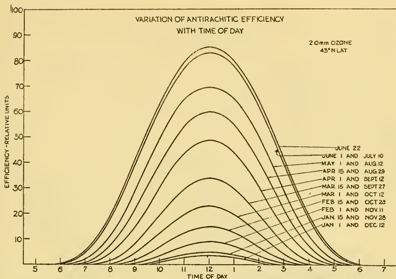
FIGURE 16.—Hourly variation of solar antirachitic effect. (2.0 mm. zenith ozone, 43° N. latitude.)
