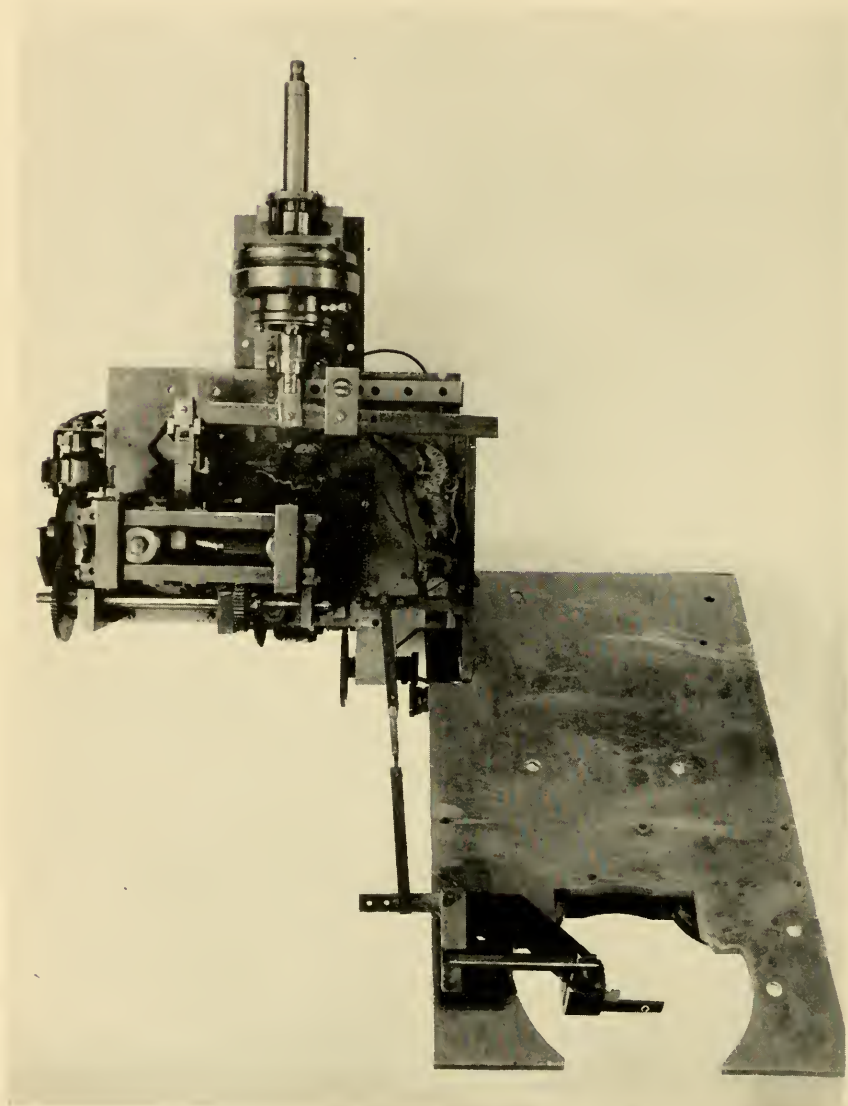
DIAPHRAGM PUMP INJECTOR OF VARIABLE THROW GOVERNED BY DIFFERENTIAL HEAT EXPANSION BETWEEN BOILER AND INVAR TAPE. Rollers which support the mirror seen behind the aluminum plate.
