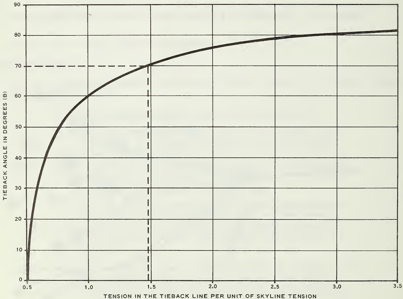
Figure 5-4 - Relative tieback load vs. tieback angle.
