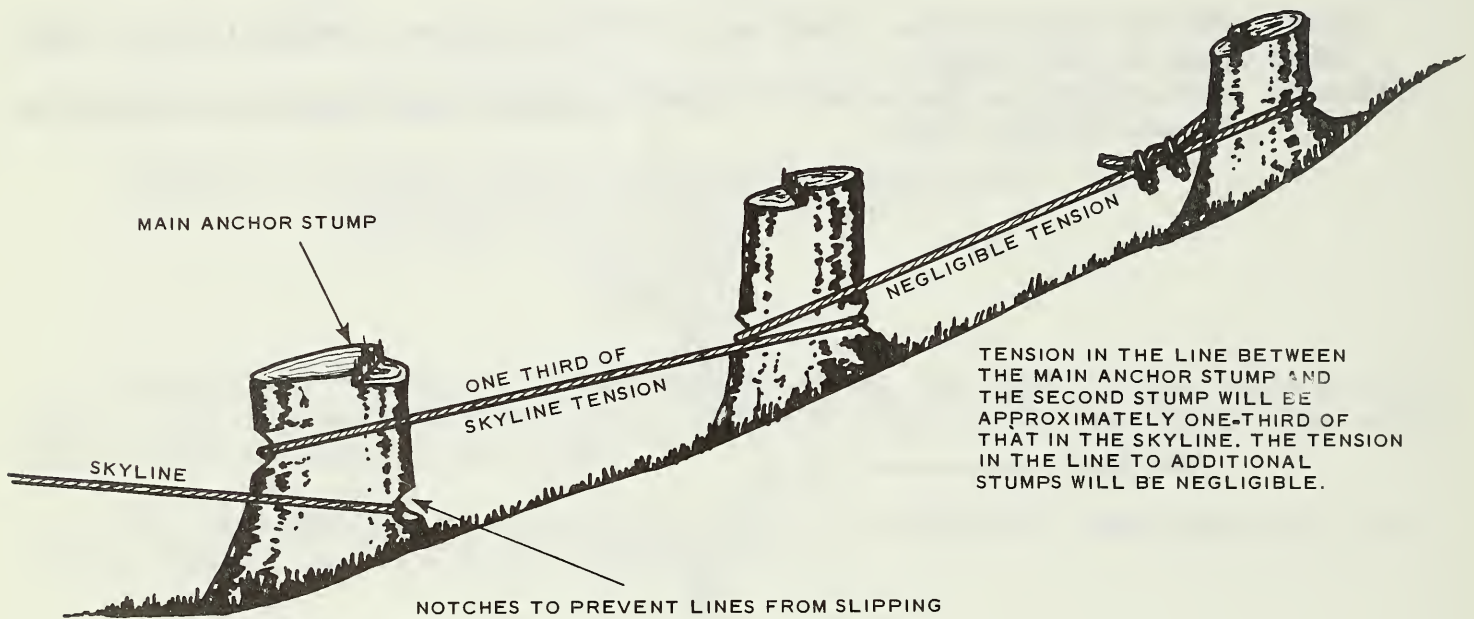
Figure 5-7. - Profile of common three-stump anchor.
