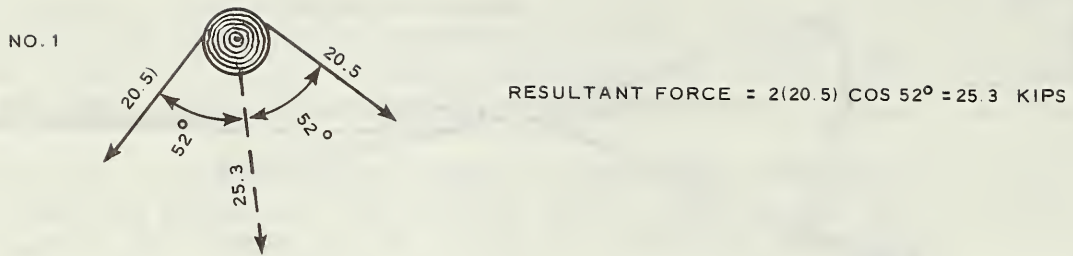
Figure 5-12c. - Resultant force on stump No. 1
