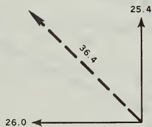
Figure 5-9d. - Resultant load diagram.
