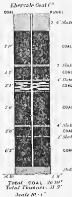
Mine Sheet No I BIG BLACK CREEK BASIN EBERVALE COLLIERY MAMMOTH BED
