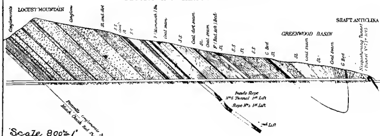
SECTION N°7 THROUGH TUNNEL N°7
