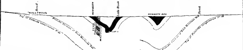
LITTLE BLACK CREEK BASIN, SECTION N° 14, THROUGH HOLLYWOOD WORKINGS.
