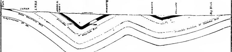
BIG BLACK CREEK BASIN. SECTION No 17, THROUGH JEDDO SLOPE No 3 AND WORKINGS.
