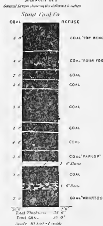
No 19 Mine Sheet No II LITTLE BLACK CREEK BASIN MILLSVILLE COLLIERY MAMMOTH BED
