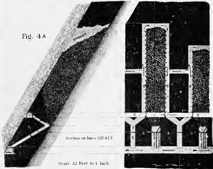
SINGLE SHUTE BREAST WITH BATTERY STEEP DIP.
