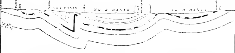
POND CREEK BASINS - POND CREEK COLLIERY:
