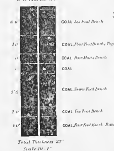
No 283 Mine Sheet No I LITTLE BLACK CREEK BASIN JEDDO COLLIERY MAMMOTH BED GENERAL SECTION SHOWING THE DIFFERENCE BETWEEN G. R. March & Co
