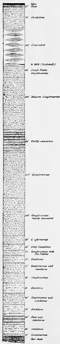
POTTSVILLE CONGLOMERATE MERQUEMONG GAP FROM MAUCH CHURCH BED SHALE No. 32 TO THE 1ST COAL BED IN TUNNEL No. 1
