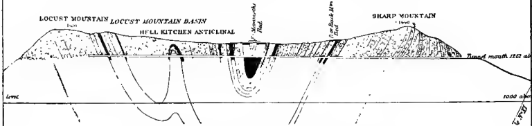
SECTION N°2 THROUGH RHUME RUN (N°1) TUNNEL.
