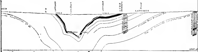
LITTLE BLACK CREEK BASIN, SECTION N° 10, THROUGH WORKINGS OF LATTIMER SLOPES N° 1 AND 2
