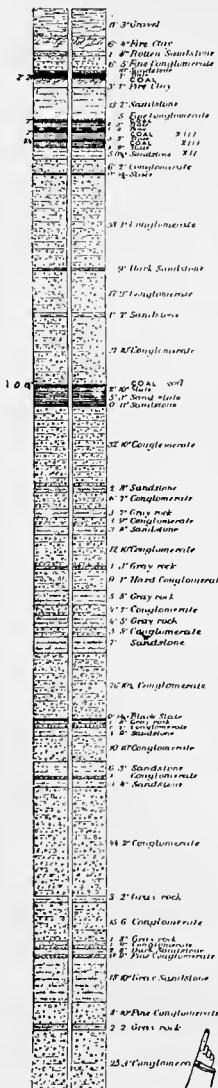
DIAMOND DRILL BORE HOLE No 4 1200' SOUTHEAST OF ALTA MOUNT COLLIERY No 2
