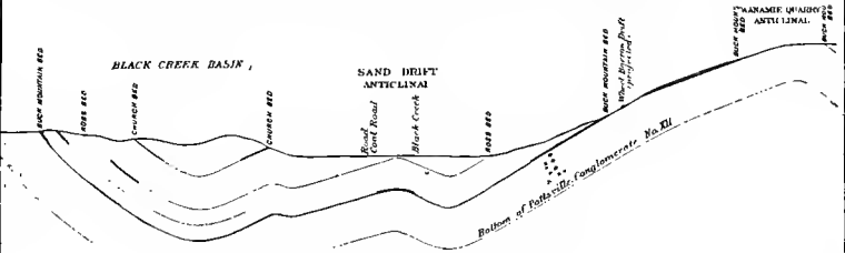
THROUGH THE MINE WORKINGS OF SALEM COLLIERY (SALEM COAL CO.)
