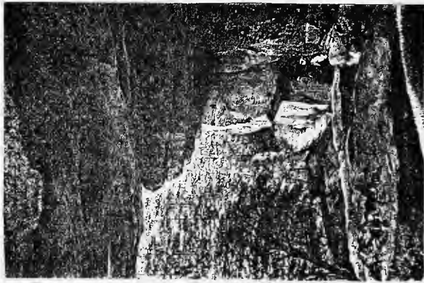
DINING HALL PASS, OLEAN, ROCK CITY
