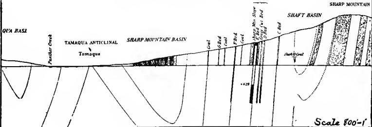
SHARP MOUNTAIN GAP AT TAMAQUA.
