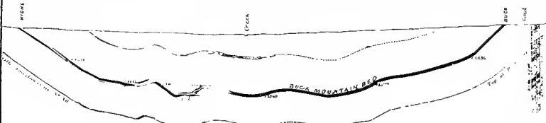
CROSS CREEK BASIN SECTION No. 6 THROUGH HIGHLAND SLOPE No. 1 AND No. 2 WORKINGS
