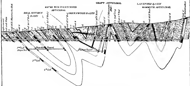
SECTION N°3 THROUGH TUNNEL N°2.
