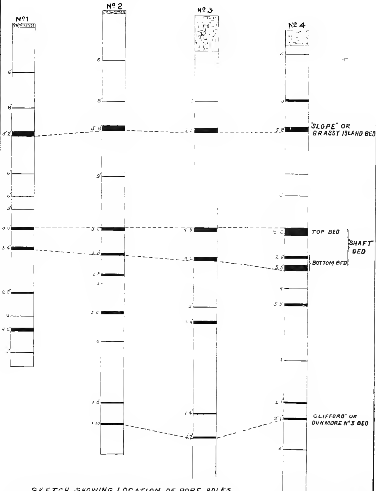
SKETCH SHOWING LOCATION OF BORE HOLES
