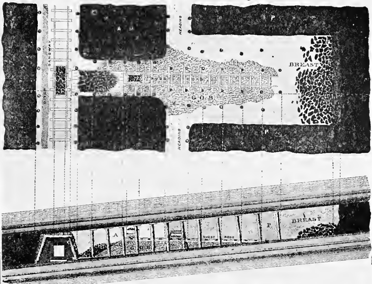
Fig. 4. SINGLE SHUTE BREAST. Flat workings with Buggy
