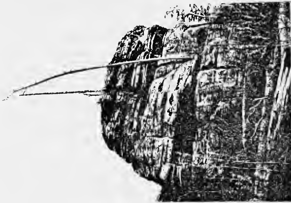
THE OLEAN CONGLOMERATE AT THE ROCK CITY CATARAUGUS CO. N.Y.
