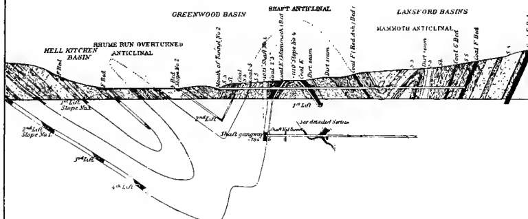
SECTION N°7 THROUGH TUNNEL N°7
