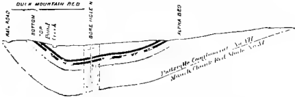
CROSS CREEK BASIN - SECTION No. 33 ON MINE SHEET No. V THROUGH SANDY RUN COLLIERY.
