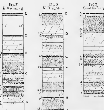
Three Sections of the Lower Productive Coal Measures in Western Pennsylvania.
