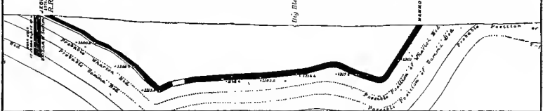
BIG BLACK CREEK BASIN. SECTION No 18, THROUGH EBERVILLE SLOPE No 1.
