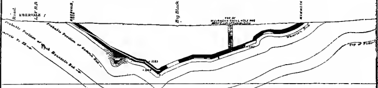
BIG BLACK CREEK BASIN. SECTION No 20, THROUGH HARLEIGH SLOPE No 3 AND WORKINGS.
