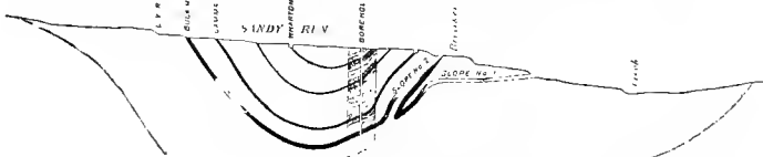
CROSS CREEK BASIN SECTION No. 6 THROUGH HIGHLAND SLOPE No. 1 AND No. 2 WORKINGS
