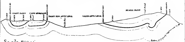
THROUGH THE MINE WORKINGS OF SALEM COLLIERY (SALEM COAL CO.)
