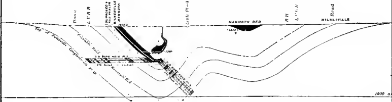
LITTLE BLACK CREEK BASIN, SECTION N° 14, THROUGH HOLLYWOOD WORKINGS.
