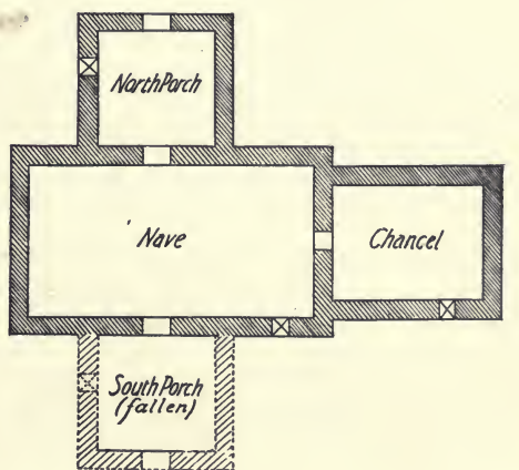
Scale PLAN OF SAXON CHURCH, BRADFORD-ON-AVON
