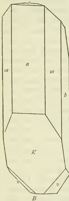
FIG. 1.—CRYSTAL OF VIVIANITE.
