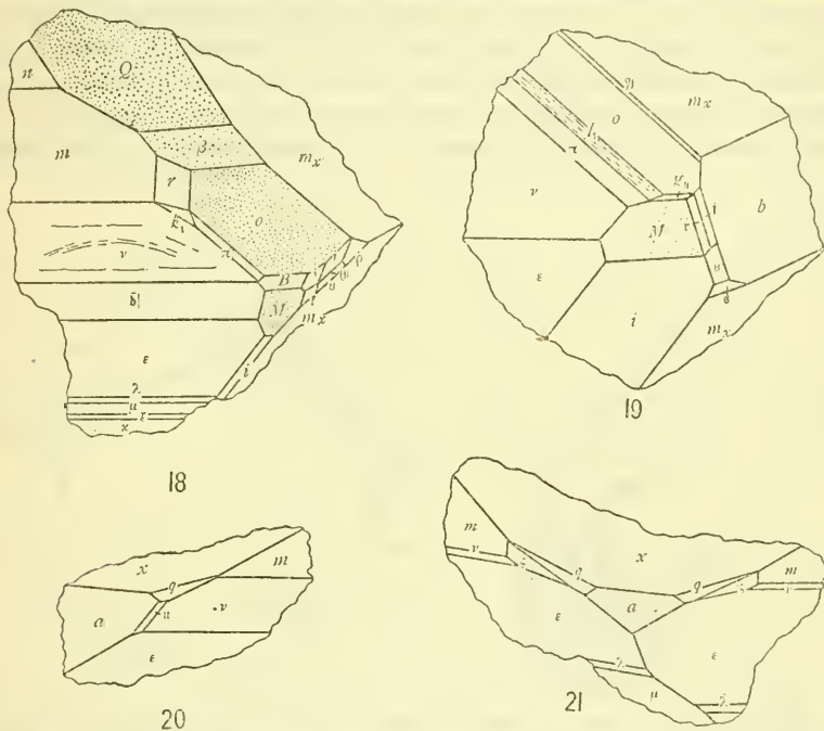
FIGS. 18-21.—18, CLINOGRAPHIC DETAIL OF CRYSTAL 41 SHOWING THE NEW FORMS k_1 ( \bar{7}94 ), i ( \bar{1}42 ), f ( \bar{1}43 ), g ( \bar{2}96 ), o ( \bar{2}95 ), \beta ( \bar{2}.10.5 ), AND r ( \bar{2}29 ). 19, CLINOGRAPHIC DETAIL OF CRYSTAL 10 SHOWING RARE AND NEW FORMS \vartheta ( 6.15.2 ), l_1 ( 9.16.2 ), g_1 ( \bar{2}62 ), r ( \bar{2}32 ), i ( \bar{2}42 ), g ( \bar{2}96 ), AND g ( \bar{2}.12.10 ). 20, CLINOGRAPHIC DETAIL OF PORTION OF CRYSTAL 44 SHOWING NEW FORM u ( \bar{2}11 ). 21, CLINOGRAPHIC PROJECTION OF CRYSTAL 43 SHOWING UNUSUAL FORM r ( 530 ).
