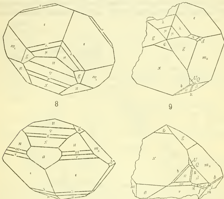
FIGS. 8-9.—8, ORTHOGRAPHIC AND CLINOGRAPHIC PROJECTIONS OF CRYSTAL 2S. AN UNUSUAL HABIT WITH THE STEEP PYRAMIDAL FORM OF TYPE 2 BUT WITH AN ORTHODOME SERIES INCLUDING \mathfrak{R} (205) AS IN CRYSTALS OF TYPE 4. 9, ORTHOGRAPHIC AND CLINOGRAPHIC PROJECTIONS OF CRYSTAL B9 SHOWING UNUSUAL PYRAMIDAL FORM WITH THE FORMS \mathfrak{h} (768), \mathfrak{R} (454), f_1 , (361), AND m_1 , (12.25.1).
