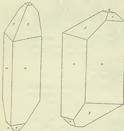
FIG. 2.—CREEDITE CRYSTAL, TYPE II.
