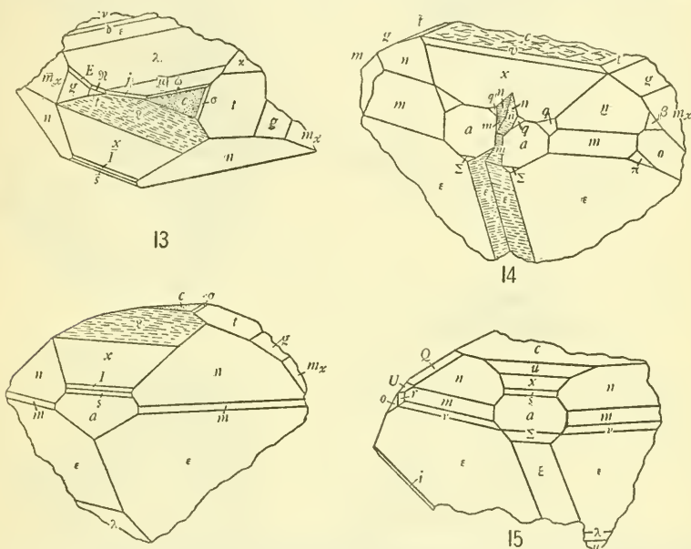
FIGS. 13-15.—13, ORTHOGRAPHIC AND CLINOGRAPHIC PROJECTIONS OF CRYSTAL B5, SHOWING UNSYMMETRICAL DEVELOPMENT, ETCHING OF c(001) , AND STRIATION OF q(205) ; ALSO THE RARE AND NEW FORMS s(302) , l(203) , \omega(\bar{1}16) , N(\bar{1}26) , E(\bar{1}38) , AND j_1(5.6.30) . 14, CLINOGRAPHIC PROJECTION OF CRYSTAL B11, SHOWING PARALLEL GROWTH WITH REENTRANT ANGLE RESEMBLING TWINNING. ALSO SHOWS CHARACTERISTIC "RULING" OF THE BASAL PINACOID. 15, CLINOGRAPHIC PROJECTION OF CRYSTAL 39 SHOWING PROMINENT DEVELOPMENT OF \Sigma(302) AND \xi(\bar{1}02) .
