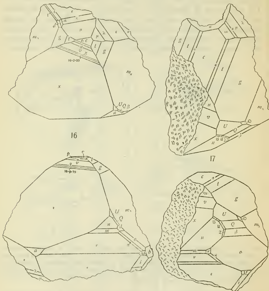
FIGS. 16-17.—16, ORTHOGRAPHIC AND CLINOGRAPHIC PROJECTIONS OF CRYSTAL 10 SHOWING FORM AND DEVELOPMENT, ALSO THE FORMS \Gamma (167) \mathcal{Q} (205) AND THE VICINAL FORM (16.0.39). 17, ORTHOGRAPHIC AND CLINOGRAPHIC PROJECTIONS OF CRYSTAL 51 SHOWING THE NEW FORMS \mathcal{Z} (343), \mathcal{U} (344), \mathcal{S} (345) AND \mathcal{D} (134).
