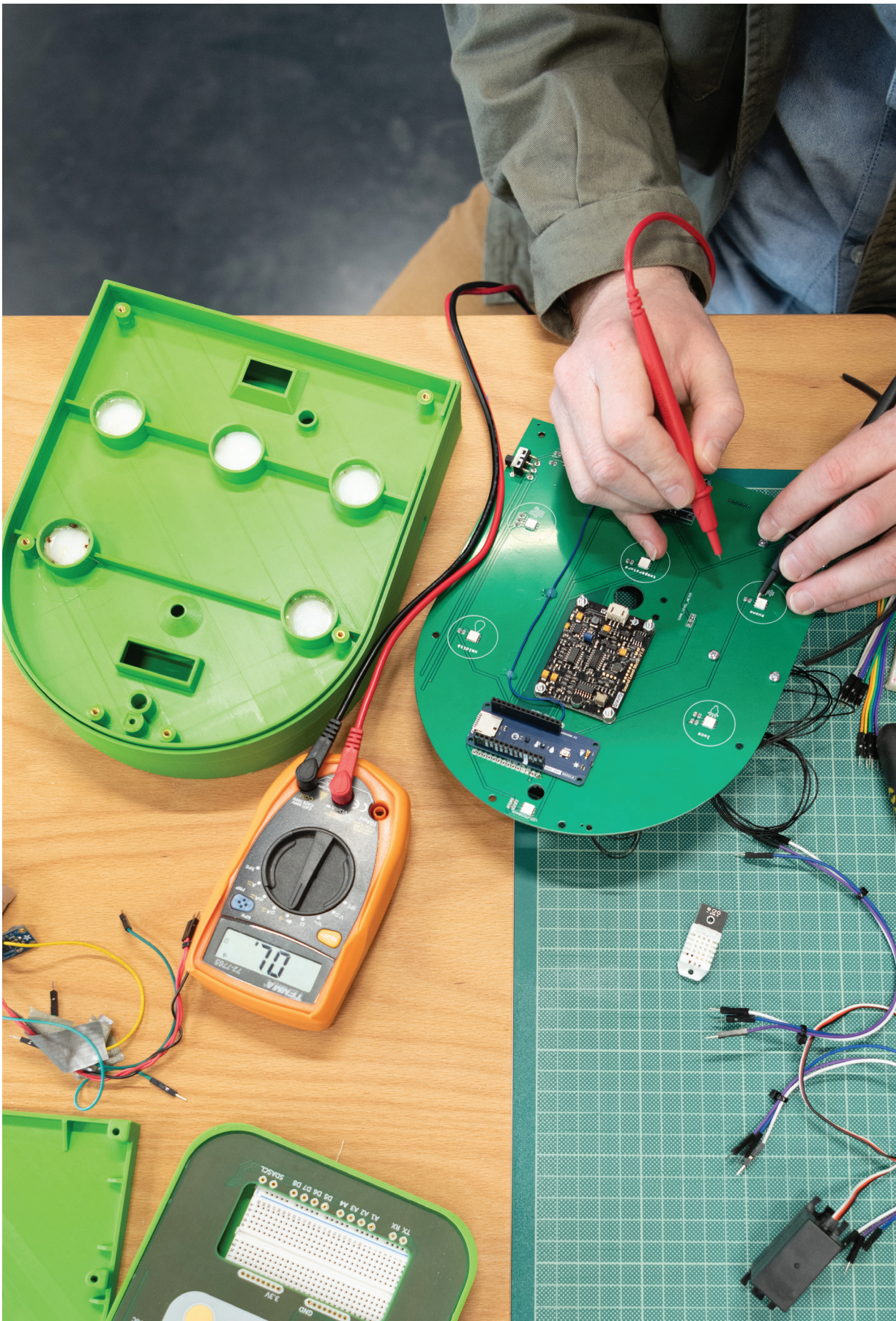
TAC Kit - Electronics
