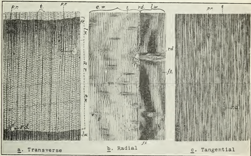
FIG. 7.— a , transverse, b , radial, and c , tangential sections of western yellow pine, magnified 20 diameters; a. r. , annual (layer) ring; e. w. , early wood; l. w. , late wood; p. r. , pith rays; r. d. , resin ducts; t. , tracheids; f. t. , flattened tracheid.
