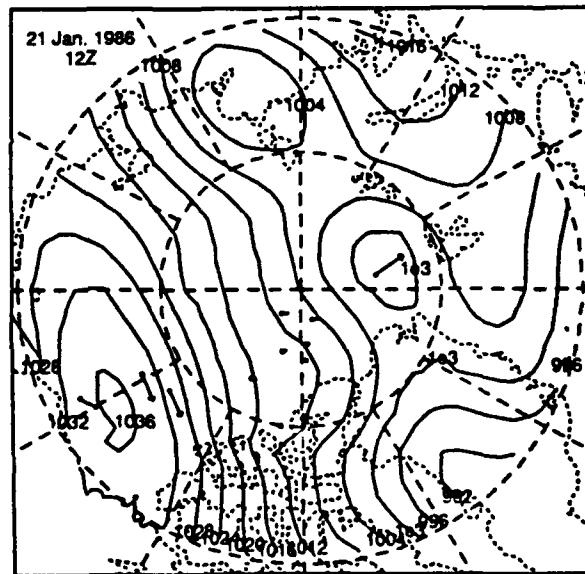
Figure 4.8 Buoy trajectories and buoy derived surface pressure for (a) 18 January, (b) 19 January, (c) 20 January, and (d) 21 January 1986. For estimation of buoy speed 1 cm equals 23.1 cm/s.
