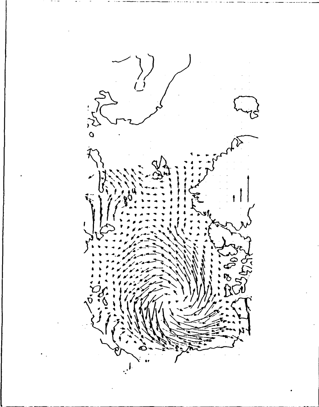
Figure 4.29 Model ice drift trajectories in cm/s for 19 August 1986. The three vectors toward the hot- tom center represent speeds of 5, 10 and 20 cm/s, respectively.
