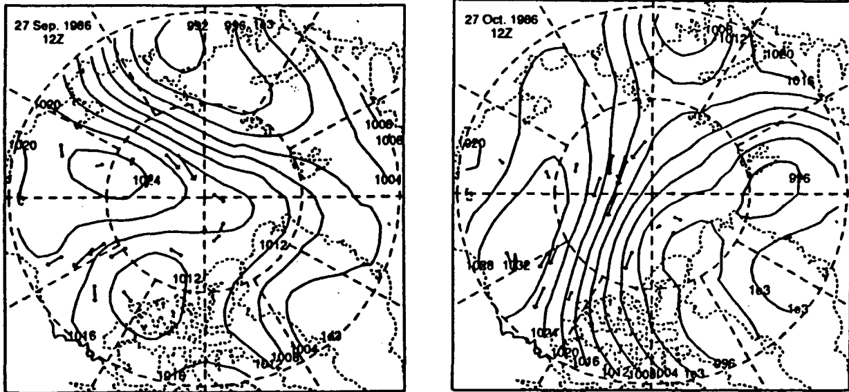
Figure 4.24 Buoy trajectories and buoy derived surface pressure for (a) 27 September, and (b) 27 October 1986. For estimation of buoy speed 1 cm equals 23.1 cm/s.
