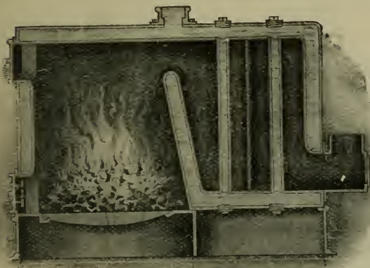
Section of WROUGHT WELDED "PAXTON" BOILER.
