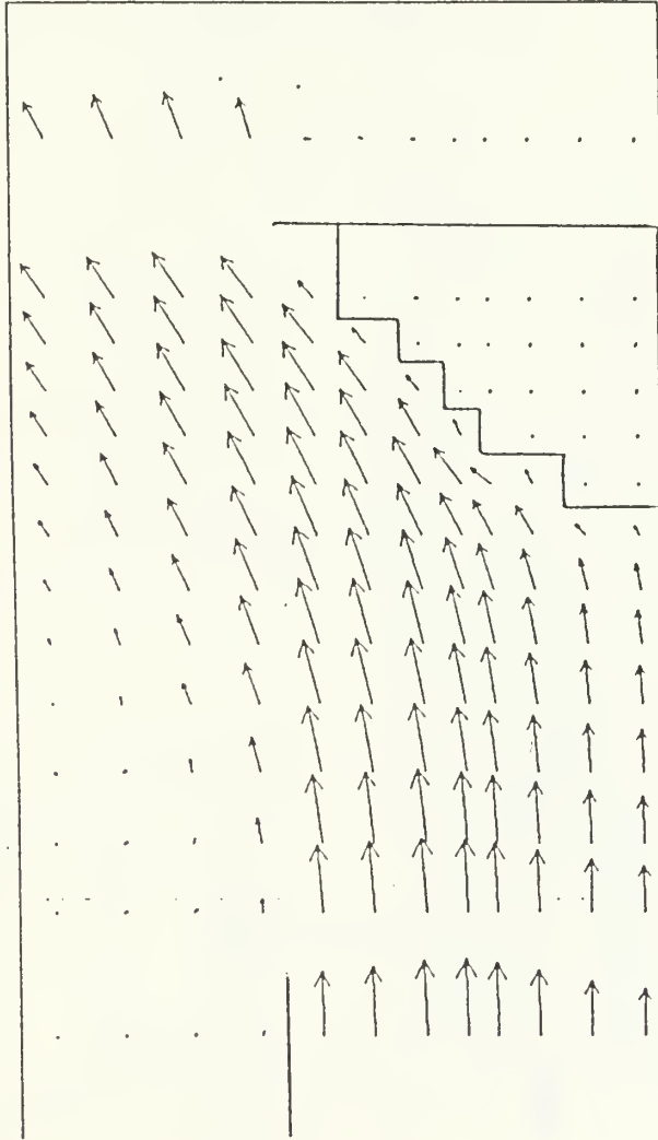
Figure 20. Velocity Vector Plot for Model 1 (exhaust)
