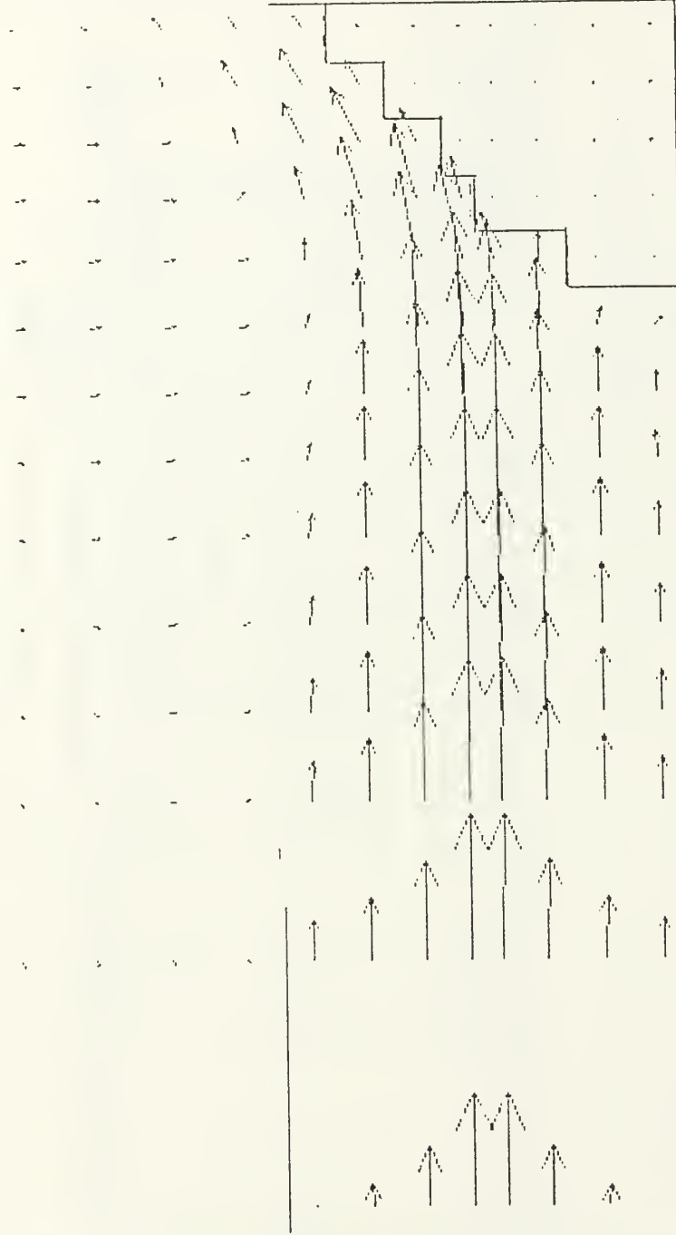
Figure 37. Velocity Vector Plot for Model 4 (exhaust)
