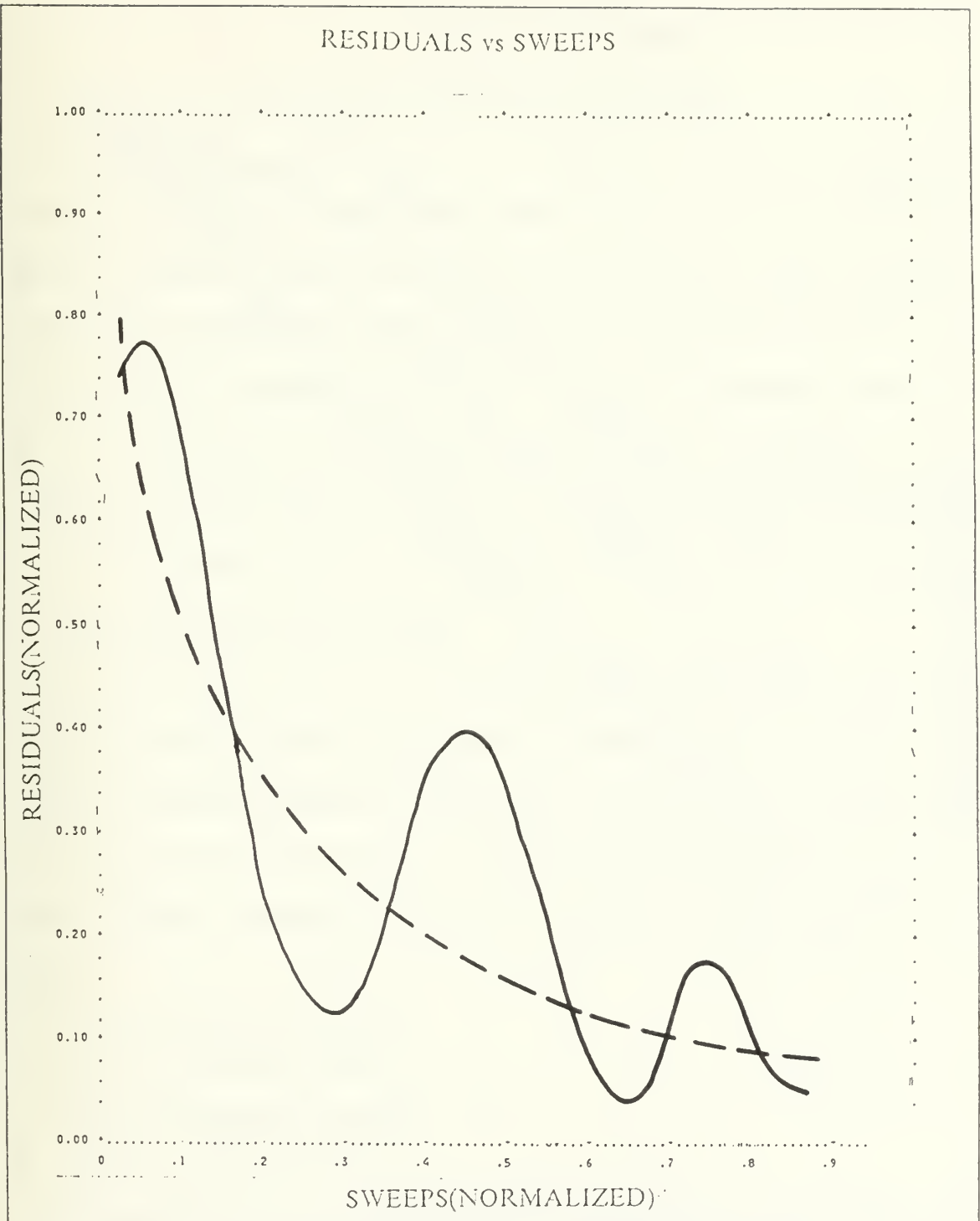
Figure 10. Sample Output Residuals vs Sweep (Converging Solution)
