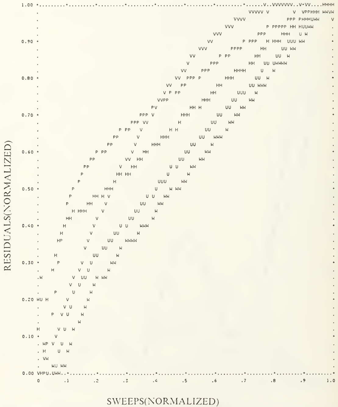
Figure 11. Sample Output Residuals vs Sweeps (Diverging Solution)
