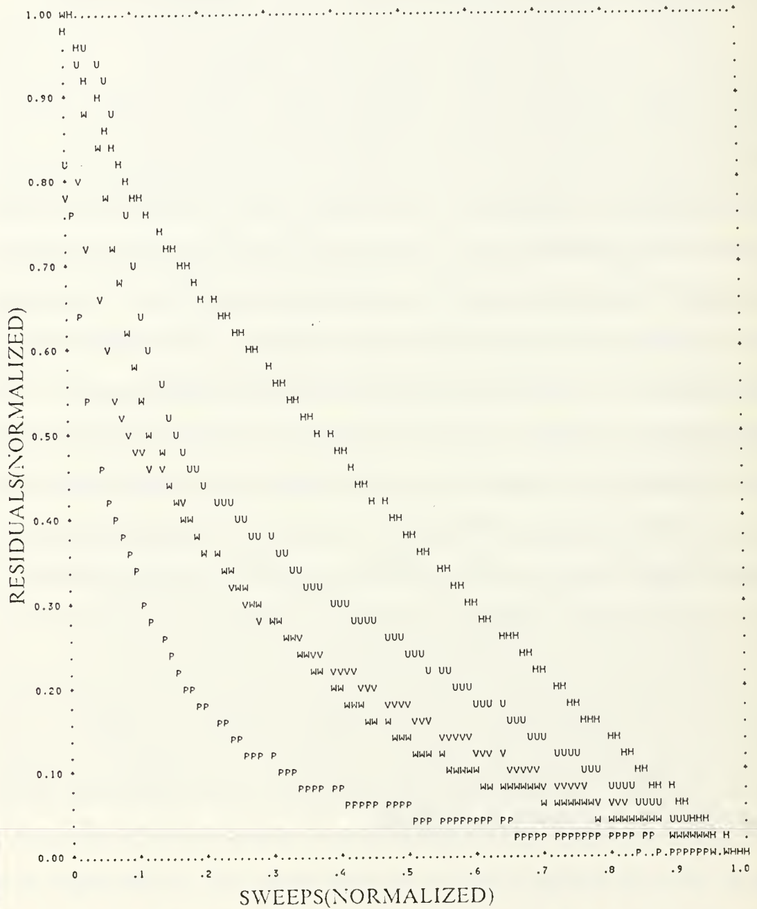
Figure 9. Sample Output Residuals vs Sweeps (Converging Solution)
