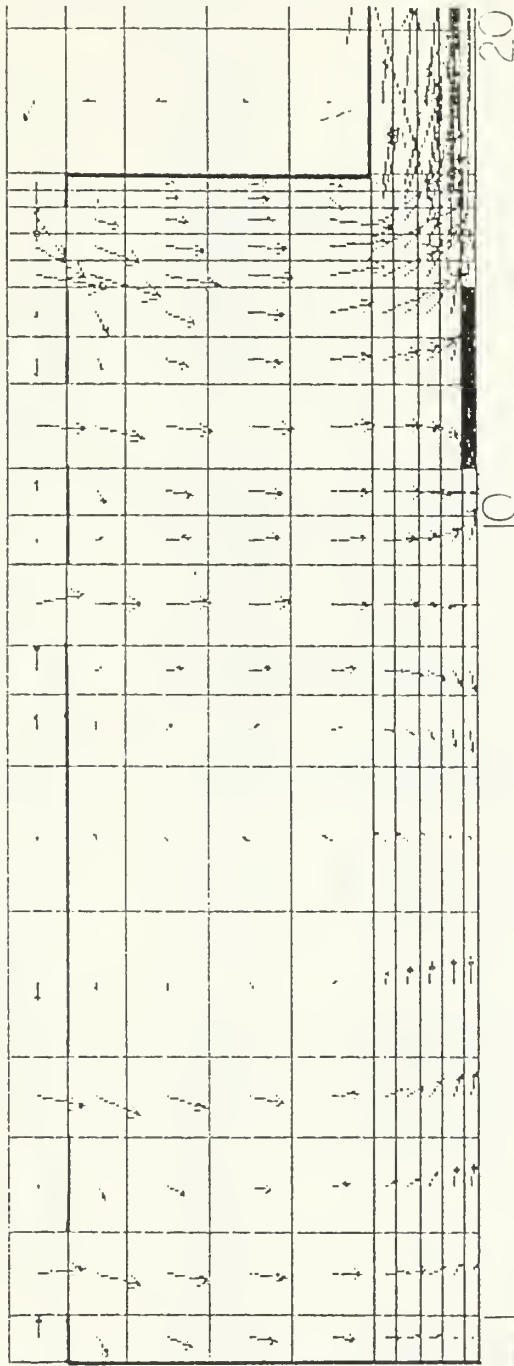
Figure 34. Velocity Vector Plot for Model 4 (test bay)
