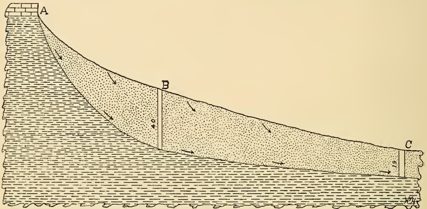
FIG. 1.—Diagrammatic section of hill at Lawrence, Kansas.
