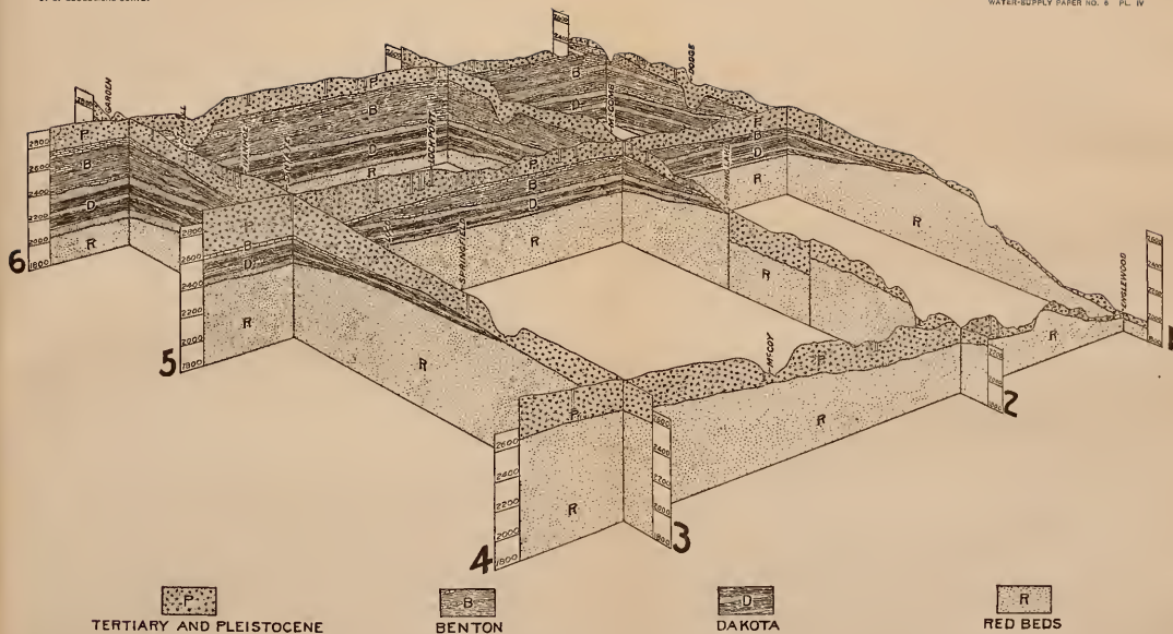
GEOLOGIC SECTIONS OF THE AREA DISCUSSED IN THIS REPORT.
