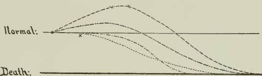
FIGURE 3.—Combined action of pilocarpine and atropine. Comparison of typical curves. See legend of Fig. 4.
