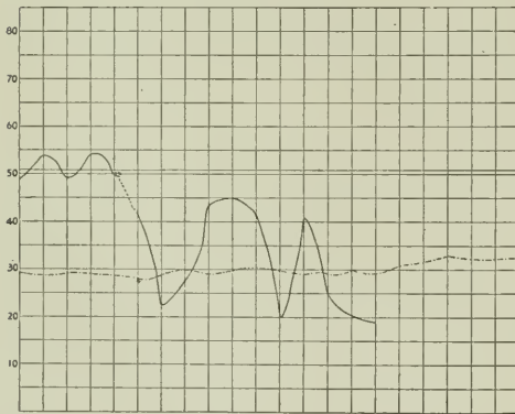
FIGURE 3.—The upper curve is from a normal animal; mean, about 51; the lower from an animal with ganglion removed; mean, 30; * marks 1 : 1000 nicotin.
