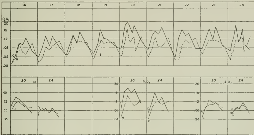
FIGURE 2. — In Fig. 2 the upper pair of curves represent the actual rate of excretion of phosphates for each subject. The ordinates represent the rate of excretion in grams per hour, the abscissæ, periods of time. The one-day curves on the 20th and 24th represent the rate of excretion of nitrogen, sulphates, and phosphates as measured by three hour periods, the same as used on all the other days. The regular curves represent, on these days only, periods of one and one-half hours.
