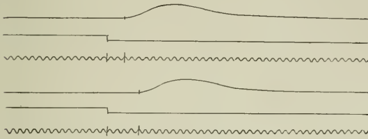
FIGURE 5.—Tracings of the contractions of the gill sac on the stimulation of the vagus near the cranium and near the gill sac. Length of nerve between the central and peripheral electrodes: 11 cm. Transmission-time: 0.046 second. Rate: 2.40 m. per second. Time: 50 d. v. per second.
