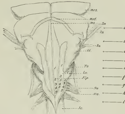
FIGURE 3. — Dorsal view of the medulla. The cerebellum removed to expose the fourth ventricle and the lobes of the medulla. The fore part of the brain was cut off at the posterior junction with the medulla. a to i , the levels employed to indicate the regions of the medulla, as a guide to the localization of function; 1 to 5 indicating where injury abolishes the function of the corresponding gill arches; mcs , posterior limit of the midbrain; mcl , cut edge of the cerebellum; ms , median suture; 5n to 10n , corresponding cranial nerves; Ll , lobus lineæ lateralis; Ta , tuberculum acusticum; Lv , lobus vagi; Flp , funiculus longitudinalis posterior; Sc , spinal cord.
