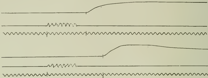
FIGURE 3.—Tracings of the contraction of the anterior part of the body on stimulation of the spinal cord in the tail and 20 cm. further anterior. Length of cord between distal and proximal electrodes: 20 cm. Transmission-time: 0.082 seconds. Rate: 2.40 m. per second.
