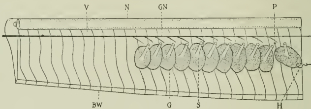
FIGURE 4. — Two-thirds natural size. Bdellostoma dobneyi . Right anterior half of body, showing relation of the vagus to the gill sacs. BW , body wall; G , gills; GN , gill nerves; H , hook serving for attachment of the thread to the recording lever; N , notocord; P , pin by which one edge of the gill sac was fixed to the board; S , sinus connecting the gill sac with the œsophagus; V , vagus nerve.
