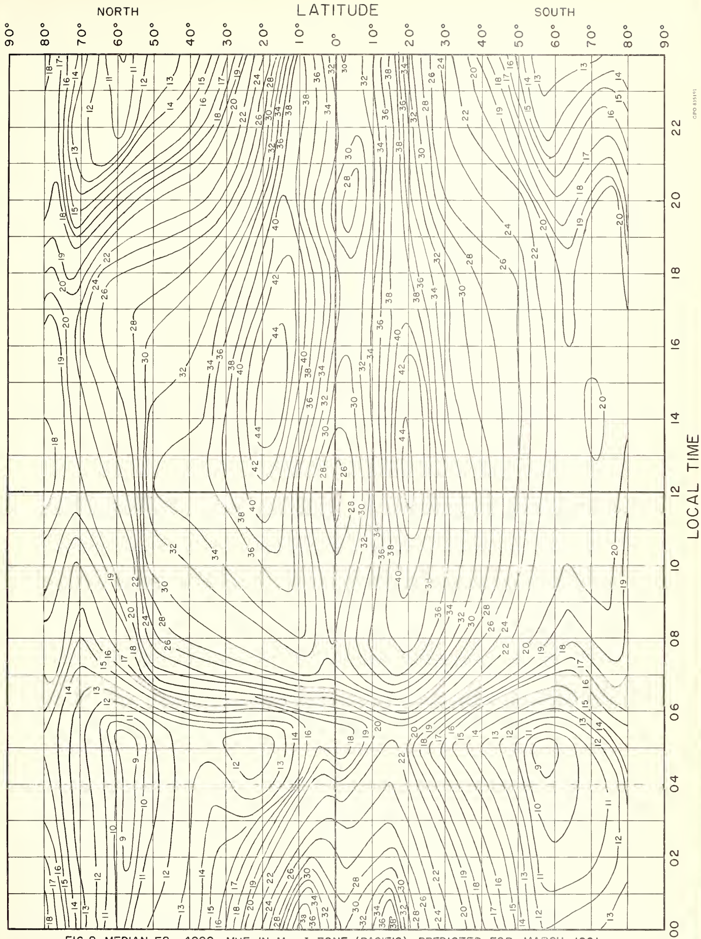
FIG. 8. MEDIAN F2 - 4000 - MUF, IN Mc, I ZONE (PACIFIC), PREDICTED FOR MARCH 1961
