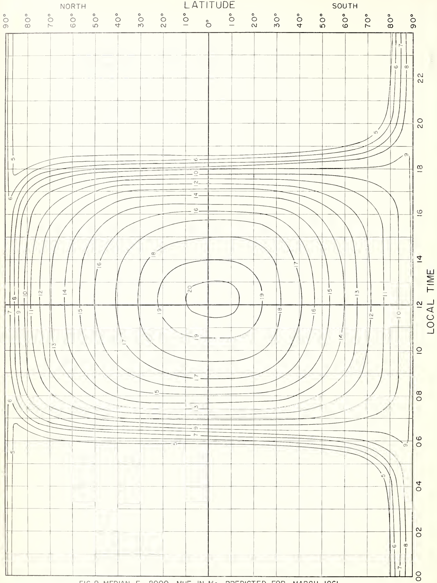
FIG. 9. MEDIAN E - 2000 - MUF, IN Mc, PREDICTED FOR MARCH 1961
