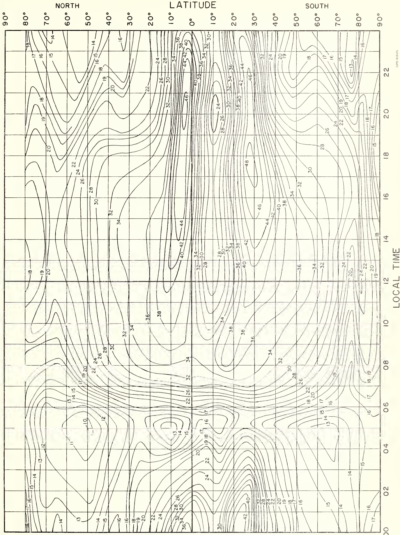
FIG. 2. MEDIAN F2 - 4000 - MUF, IN Mc, W ZONE, PREDICTED FOR MARCH 1961
