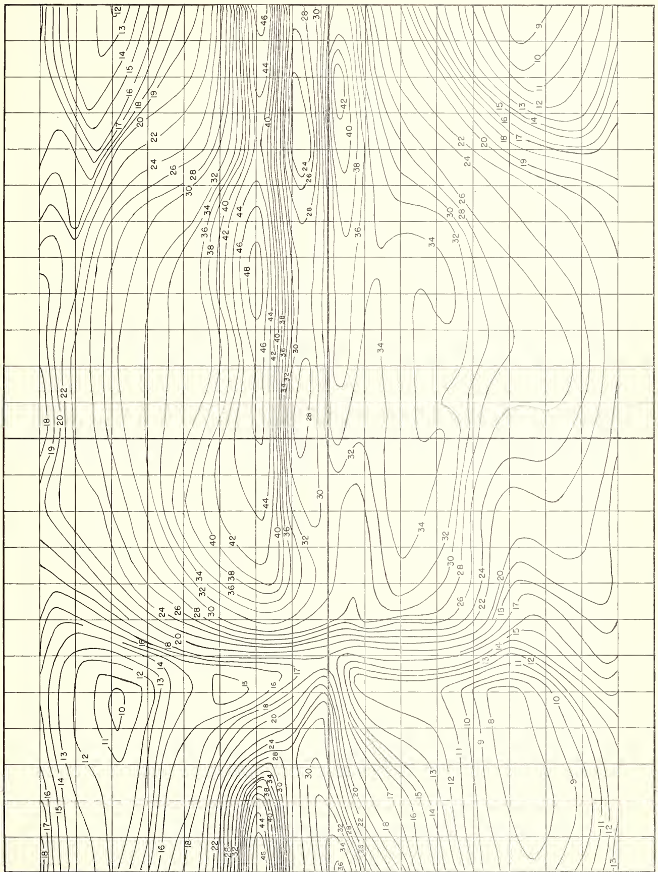
FIG. 4 MEDIAN F2 - 4000 - MUF, IN Mc, I ZONE (AFRO - EUROPEAN), PREDICTED FOR MARCH 1961
