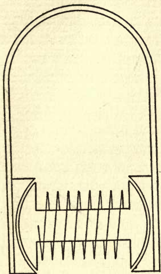
POSITION OF CORE WHEN MAGNETIZED
