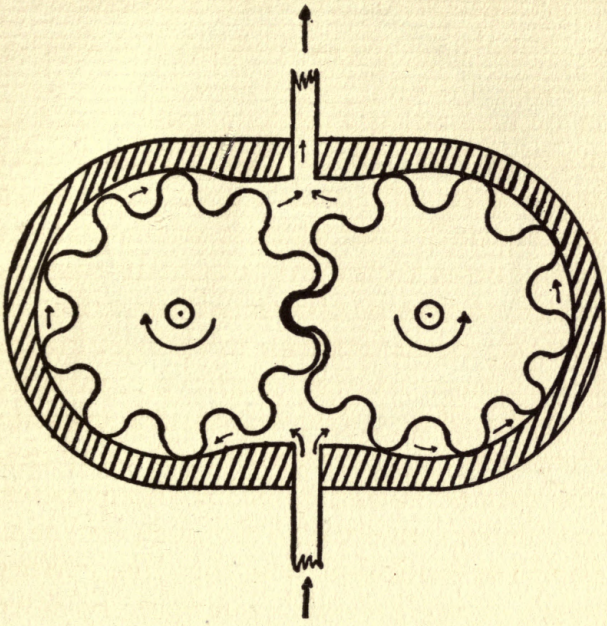
GEAR PUMP
