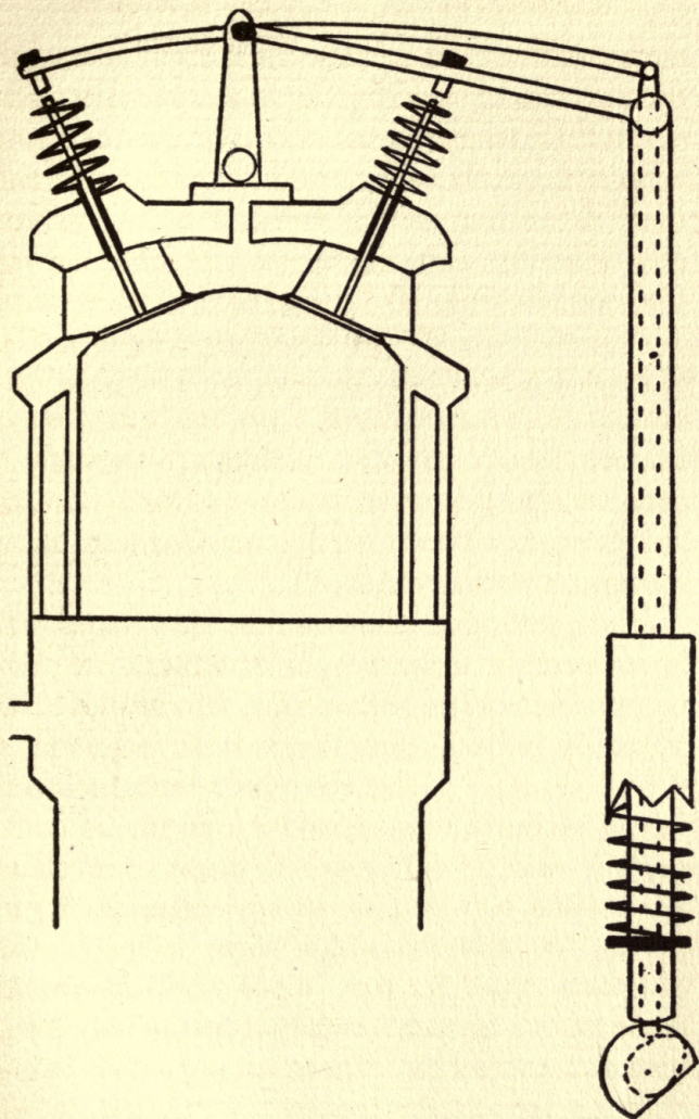
DIAGRAM TO ILLUSTRATE THE CURTISS OX VALVE ACTION
