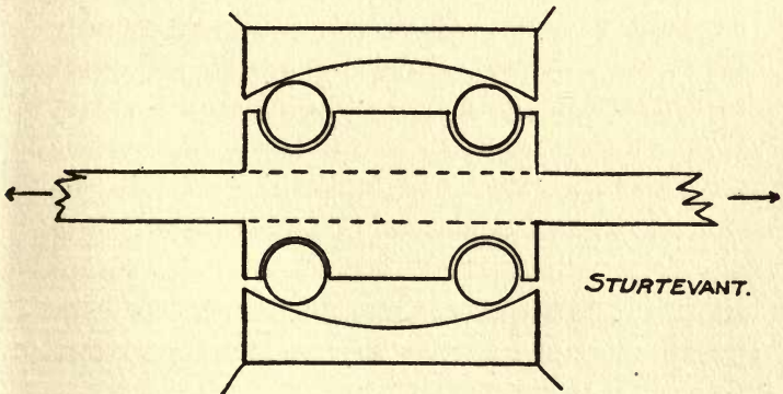
THRUST BEARINGS
