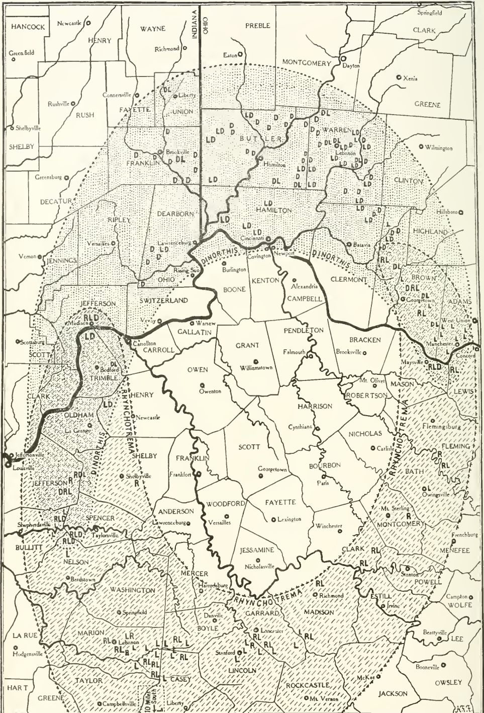
DISTRIBUTION OF DINORTIS CARLEYI , RHYNCHOTREMA DENTATA VAR., AND LEPTAENA RICHMONDENSIS VAR. IN THE ARNHEIM.
