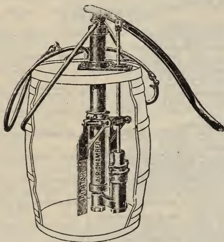
POMONA" NO. 1100, WITH AGITATOR.
