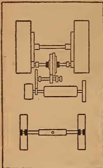
The black rectangles indicate where Timken Tapered Roller Bearings serve the Case Tractor, manufactured by the J. I. Case Threshing Machine Co., Racine, Wis.
