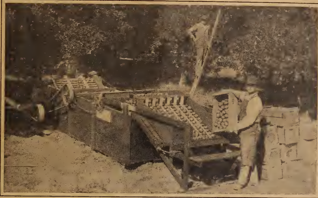
This new device, fathered by the California Fruit Growers' Exchange, tests oranges by their weight. The inferior fruit rises to the surface in the tank, the medium quality sinks part of the way down, and the good oranges go to the bottom. This machine is widely used in old American orange-growing regions
