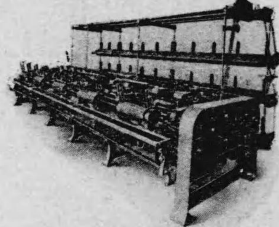
Intersecting Gill Box
