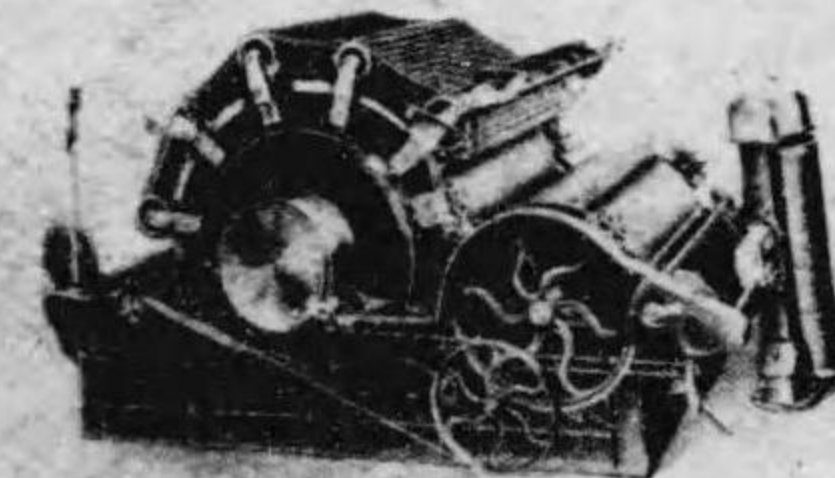
Revolving Flat Card
