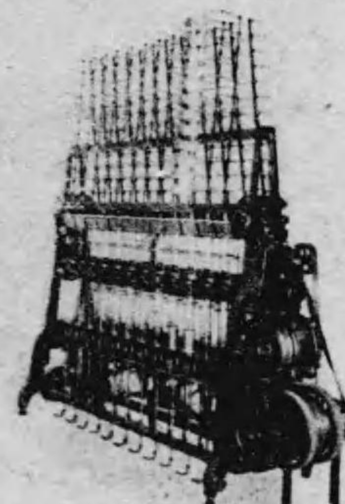
"5B" Spinner
