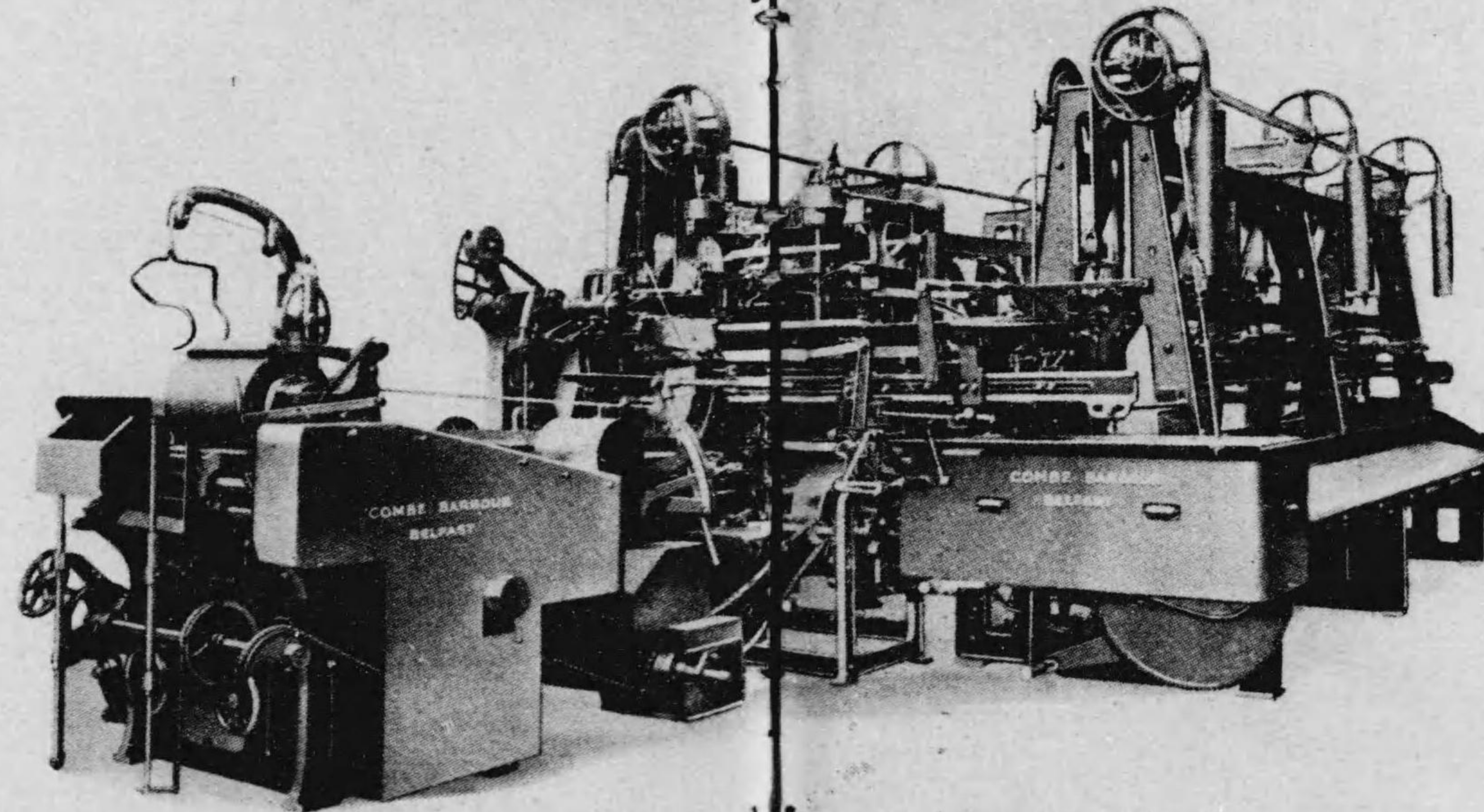
HACKLING MACHINE with Patent Transferrer and Spreadbord.
