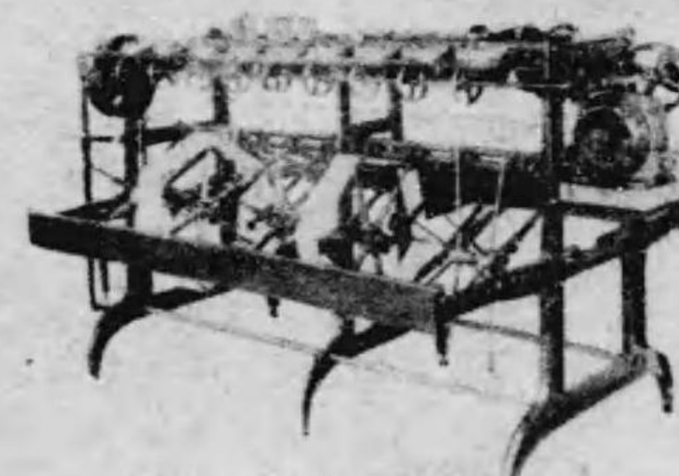
Hard Silk Winding Frame 3F Style
