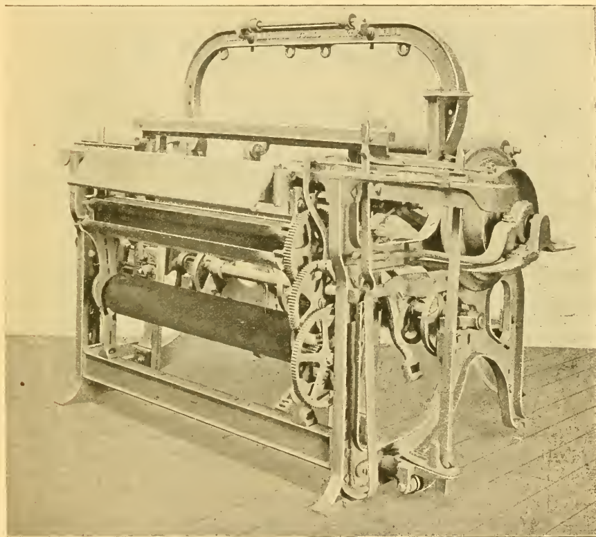
THE MASON SILK LOOM.
