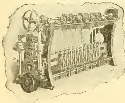
STANDARD HORSE BLANKET MACHINE.
