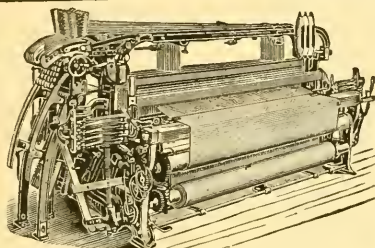
Crompton "1896" Woolen and Worsted Loom.
