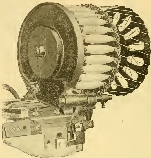
DETAIL OF HOPPER MECHANISM.
