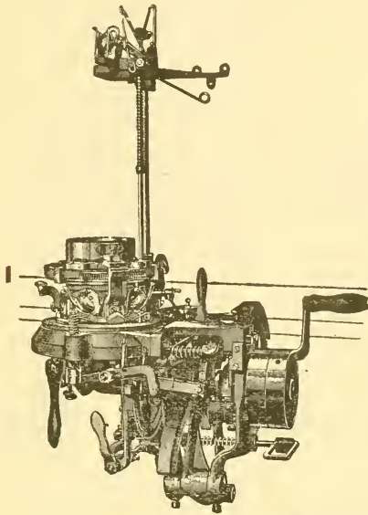
Branson 7-8 Automatic Knitting Machine.
