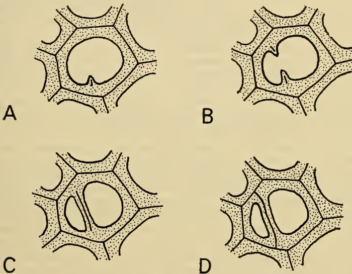
Text-fig. 1. Series of diagrammatic transverse sections showing nature of unequal, adaxial increase in Bajgolia (based on B. caespitosa ; approximately \times 11 ). A. Initial inward extension of sclerenchyme from one side of lumen only; sometimes this single protrusion extends right across lumen and is not met halfway by matching plate-like "septa" from opposite side. B-D. Stages in the development and fusion of the "septal" structures extending from both sides of the lumen to form a new dividing wall with two adjacent new "daughter" corallites.
