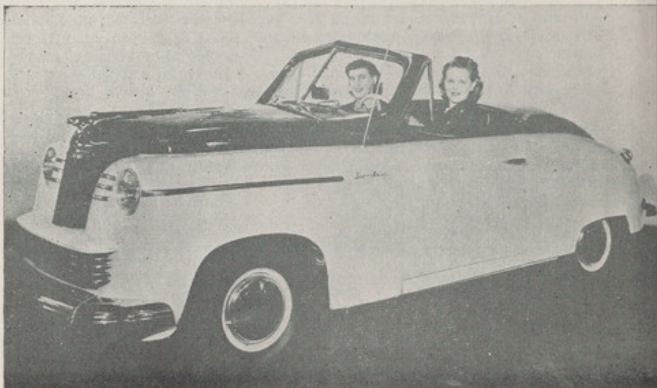
Keller "Super Chief" Convertible cradled in rubber. An unbelievable smooth ride, three passenger, 92" wheelbase, 49 h. p. engine mounted (optional) rear or front with chassis that performs like a thoroughbred.
