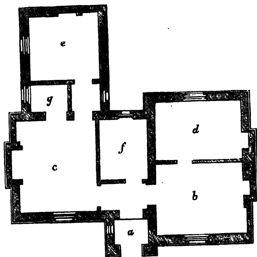
GROUND PLAN
