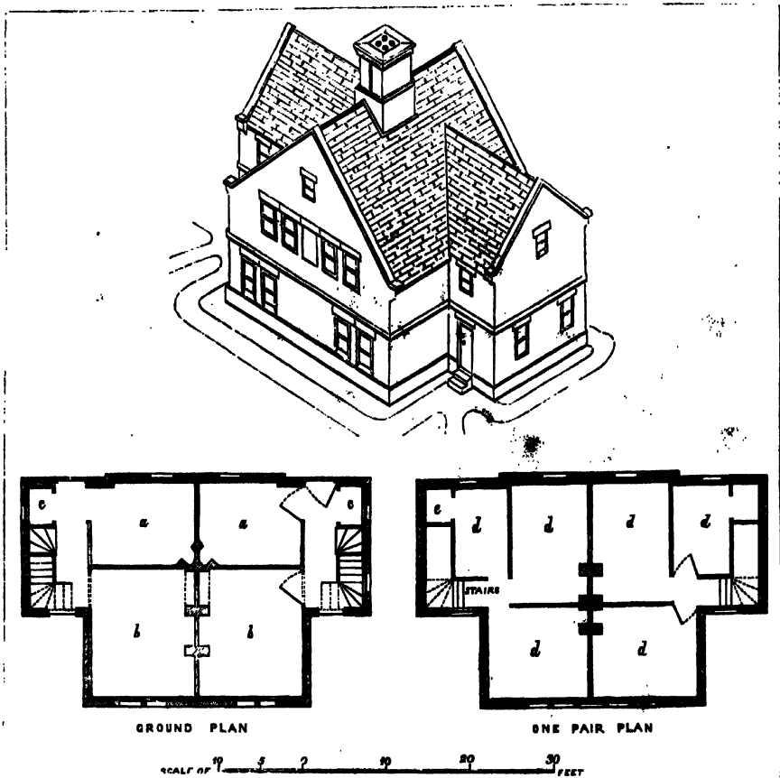
ALVERSTONE DOUBLE COTTAGE
