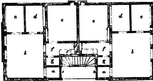
GROUND PLAN
