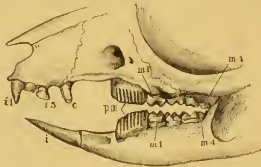
FIG. 90.—Dentition of Hypsiprymnus . i 1 to 3, three upper incisors; i , lower incisor; c , canine; pm , last upper and lower premolar; m 1 to 4, upper and lower molars.
