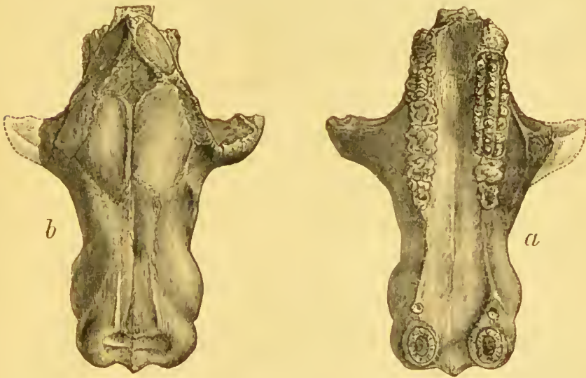
FIG. 107.—Cranium of Tritylodon longævus (Owen), Trias, Basutoland, South Africa. a =palatal view of skull, showing the dentition; b =view of the upper surface of the skull, \frac{3}{4} nat. size. (See Table-case, No. 14a.)
