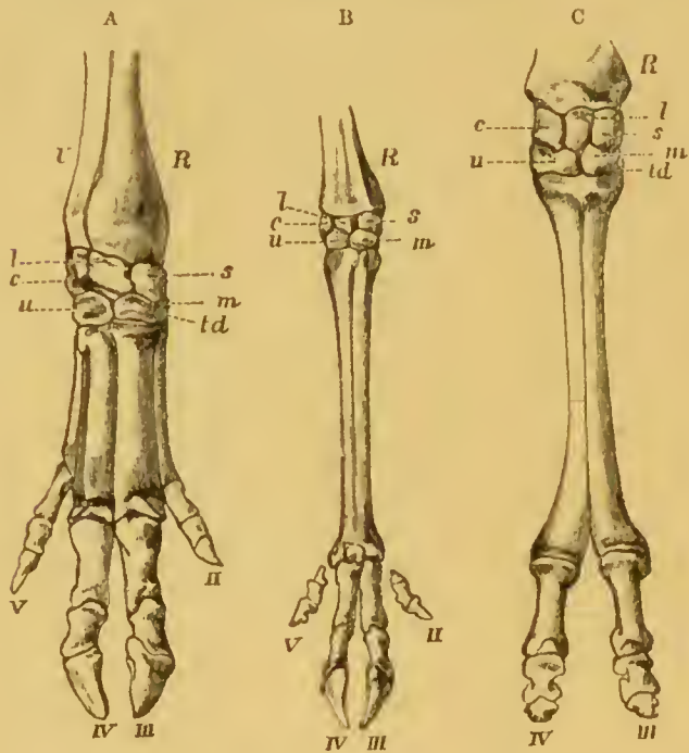
FIG. 49.—Examples of modifications of the bones in the Artiodactyle Fore-foot (after Prof. Flower). A, Pig, \frac{1}{2} nat. size. B, Deer, \frac{1}{2} nat. size. C, Camel, \frac{1}{2} nat. size. R=radius; U=ulna; c=cuneiform; l=lunar; s=scaphoid; u=unciform; m=magnum; td=trapezoid.
