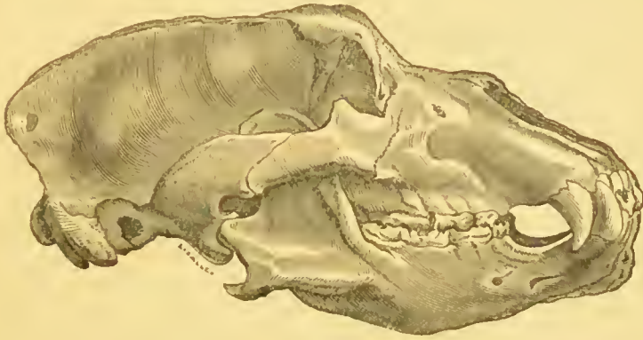
FIG. 6.—Profile of skull and lower jaw of the "Cave-Bear" ( Ursus spelæus , Rosenm.) from the Pleistocene cavern deposits of Germany (reduced).
