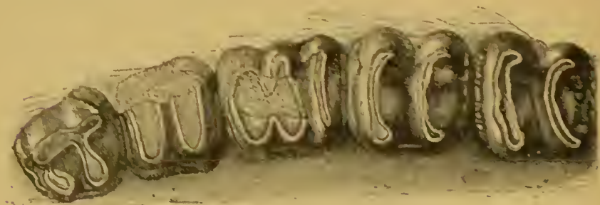
FIG. 11.—Left upper molars of Dinotherium (Kaup, \frac{1}{2} natural size; Middle Miocene, Samaran (Gers), France (after Gaudry).
