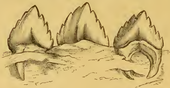
FIG. 78.—Three lower molars of Squalodon , from the Miocene of Europe.
