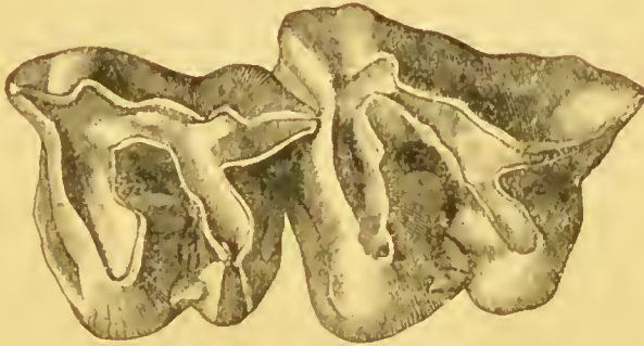
FIG. 41.—Two upper left true molars of Rhinoceros Croizeti (Fillhol), from the Upper Eocene of Bach (Dept. Lot), France.
