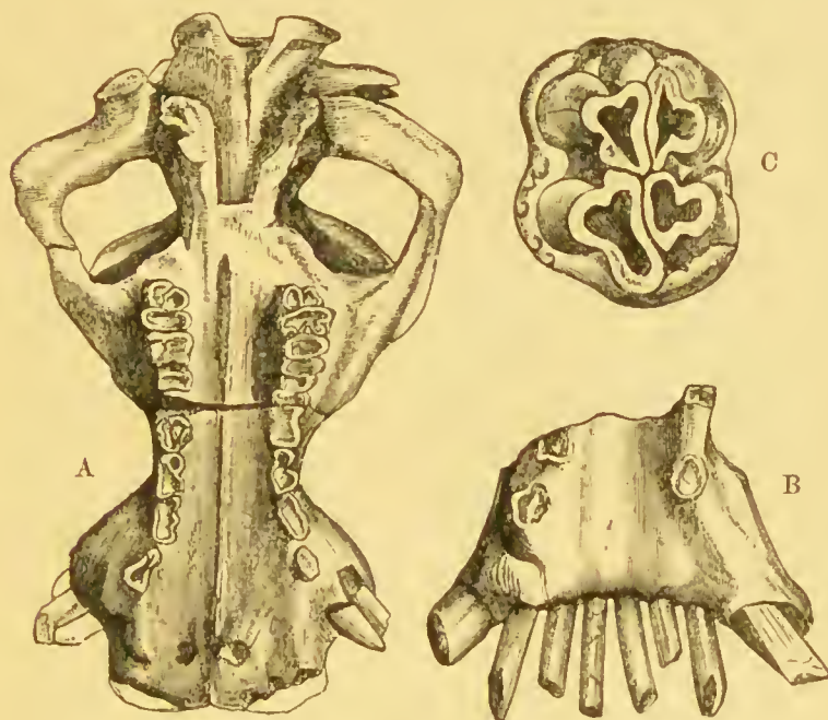
FIG. 52 A.—Palatal view of skull of Hippopotamus sivalensis (Falconer and Cautley) from the older Pliocene, Siwalik Hills, India. „ B.—Front or symphyseal portion of lower jaw of H. sivalensis , showing the six incisors and the tusk-like canines. (Both figures one-eighth natural size.) „ C.—Molar tooth of same species, showing the worn-down double trefoil pattern of the crown (one-half natural size).
