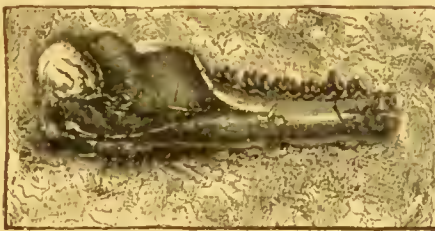
FIG. 98.—Lower Jaw and Teeth of Triconodon mordax (Owen), natural size. Middle Purbeek Beds, Dorset.
