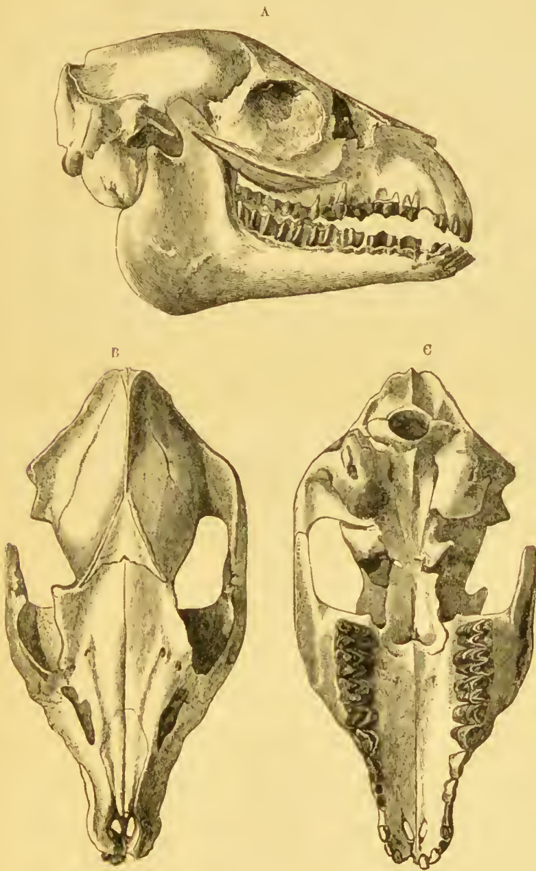
FIG. 57.—(A) Profile; (B) upper; and (C) lower, views of the skull of Cænotherium Fildholi (Lydekker). Upper Eocene, Caylux, France.
