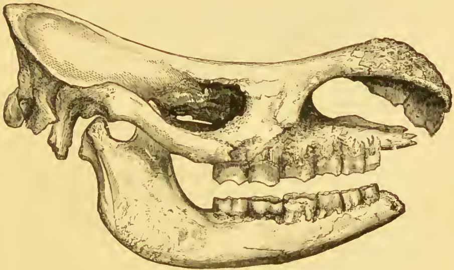
FIG. 39.—Skull and lower Jaw of Rhinoceros leptorhinus (Owen), from the Pleistocene Brick-earth of the Thames Valley, at Ilford, Essex. (See Pier-case, No. 6.)
