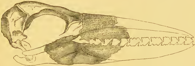
FIG. 115.—Skull of Odontopteryx toliapicus (Owen), a bird from the London Clay of Sheppey with serrated mandibles; probably a fish-eating bird, like the Merganser.
