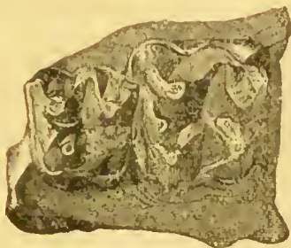
FIG. 54B.—First and second left upper true molars of Hyopotamus porcicus (P. Gervais).
