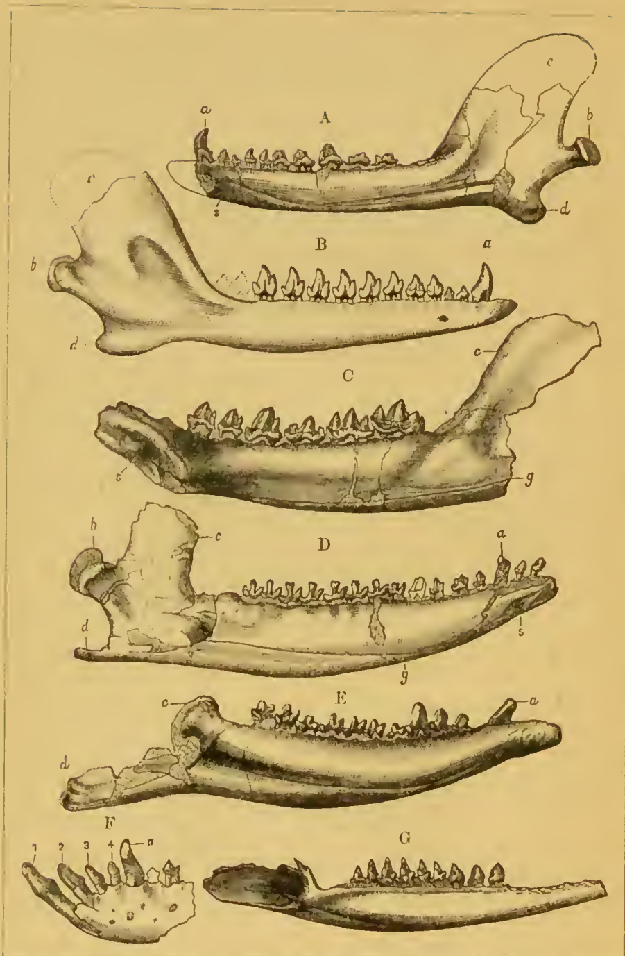
FIG. 99.—AMERICAN JURASSIC MAMMALS ( Dryolestidae ), AMPHITHERIIDÆ, AND SPALACOTHERIIDÆ, Wyoming Territory, North America.
