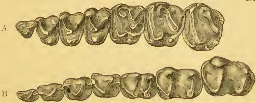
FIG. 33.—(A) the left upper, and (B) the left lower, cheek-dentition of Coryphodon hamatus (Marsh), from the Eocene of North America (from Prof. Marsh's Monograph of the Dinocerata).
