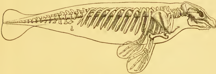
FIG. 73.—Skeleton of the living "Manatee" ( Manatus americanus ), from the River Amazon.
