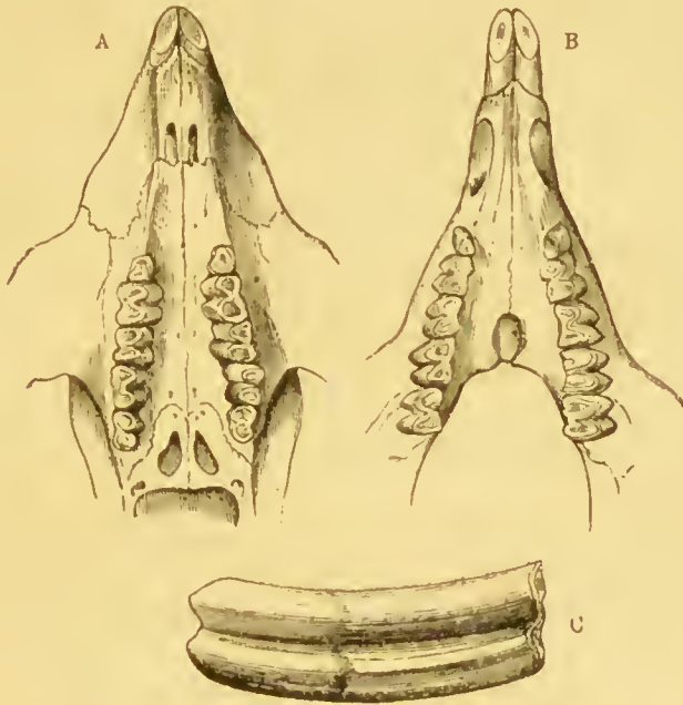
FIG. 100.—Dentition of Wombat, Phascolomys .
