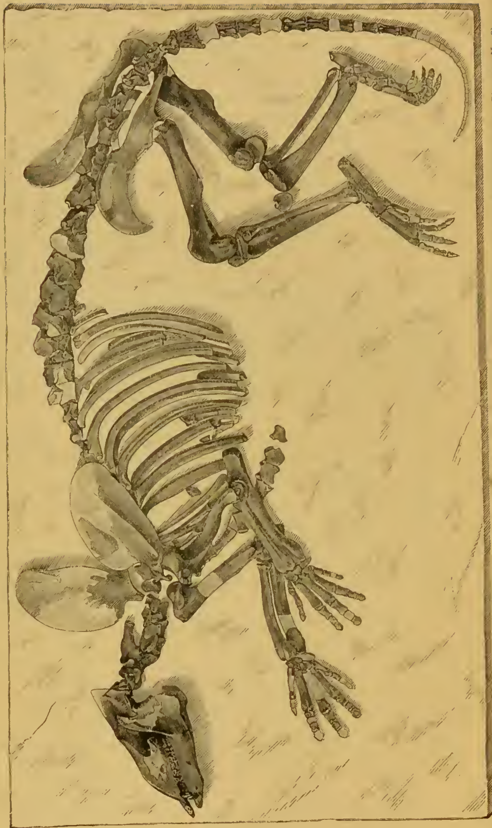
FIG 36.—Skeleton of Plioceros pricornis (Cope). Wasatch Eocene, Big-Horn Basin, Northern Wyoming, U. S. N. America. \frac{1}{4} th nat. size (see Pierce, No. 9).
