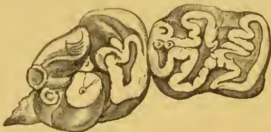
FIG. 72.—The penultimate and last lower molars, right side, of Halitherium fossile (Blainville), Middle Miocene, Angers (Maine-et-Loire), France.
