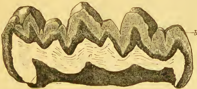
FIG. 23.—Vertical longitudinal section of the first lower true molar of Mastodon angustidens (Cuvier), from the Middle Miocene of Simorre, France; b enamel; c dentine ( \frac{1}{3} nat. size).
