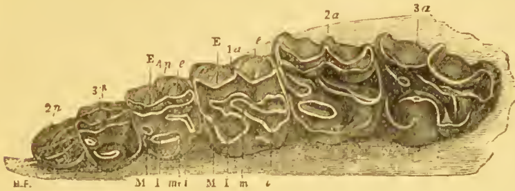
FIG. 46.—The left maxilla, with the cheek-dentition of Palaeotherium annectens . (Owen); from the Upper Eocene of Hordwell, Hampshire. 1p, 2p, 3p, 4p. = premolars; 1a, 2a, 3a, true molars; E, e, outer, I, i, inner, and M, m, middle columns, (after Gaudry).
