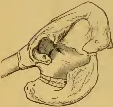
FIG. 30.—Profile of skull of Elephas planifrons (Falc. and Cautl.) ( \frac{1}{10} natural size); Older Pliocene, Siwalik Hills, India.
