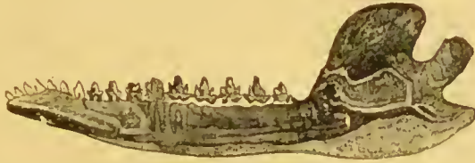
FIG. 96.—Lower Jaw and Teeth of Amphilestes Broderipii (Owen), (twice natural size), Great Oolite, Stonesfield, Oxfordshire.
