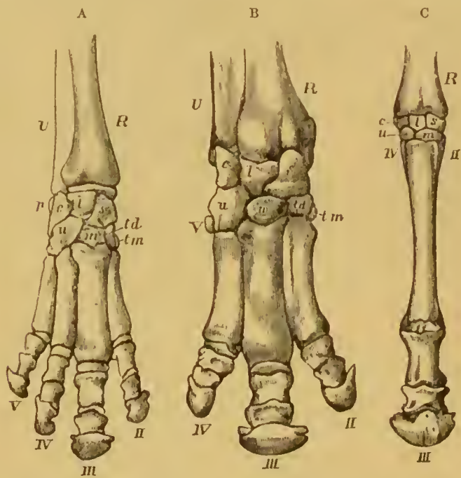
FIG. 38.—Examples of modifications of the bones in the Perissodactyle Fore-foot (after Prof. Flower).†
