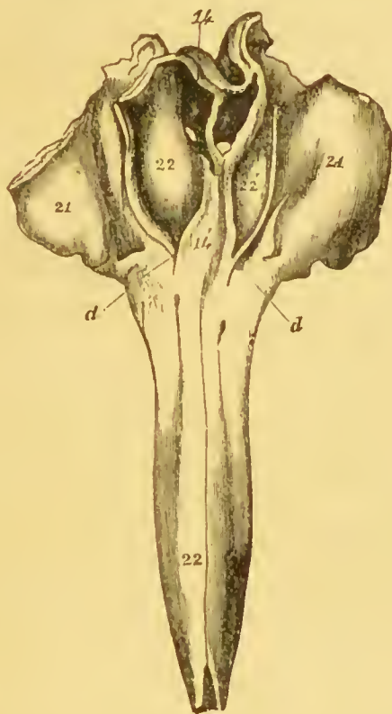
FIG. 80.—Anterior portion of cranium of Choneziphius planirostris (Cuvier), Pliocene, Antwerp Crag; \frac{1}{4} nat. size. 14', vomer; 14, mesethmoid; 21, maxilla; 22, premaxilla; d, d , canals, which terminate in the prenasal fossæ.
