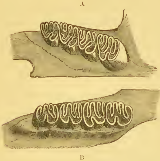
FIG. 9.—Dentition of Beaver, Castor europæus (Owen). A the left upper, B the right lower molar series. Pleistocene, Cambridgeshire Fens.
