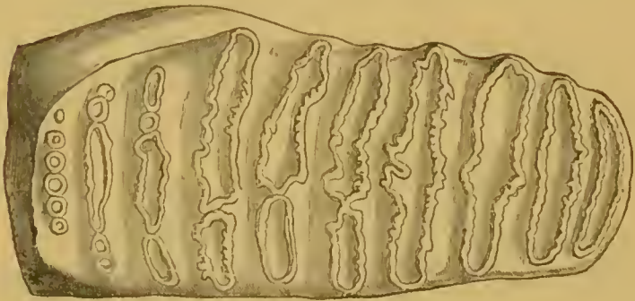
FIG. 20.—View of the grinding-surface of upper molar of Elephas meridionalis (Nesti), \frac{1}{3} natural size; from the Upper Pliocene of Tuscany.
