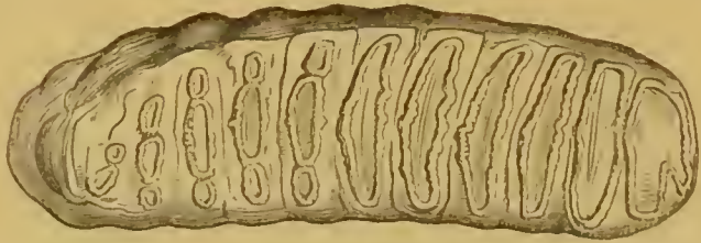
FIG. 19.—View of the grinding-surface of the second right lower true molar of Elephas antiquus (Falc.), \frac{1}{3} natural size; from the Pleistocene of Grays, Essex.
