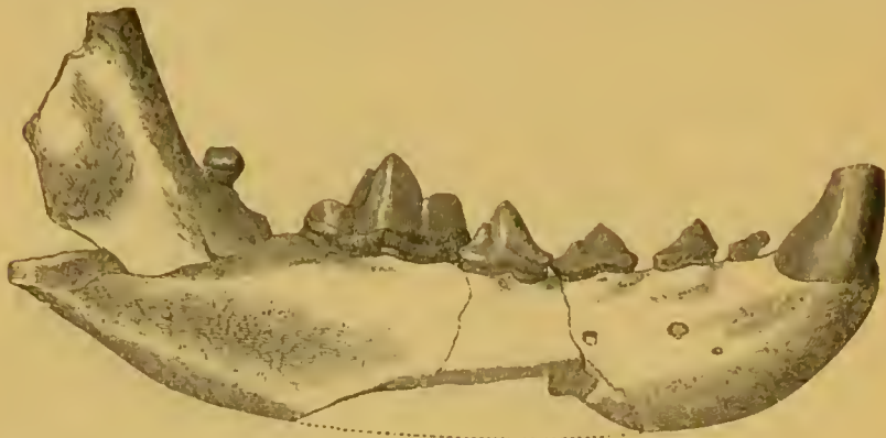
FIG. 5.—Right ramus of mandible of Cephalogale brevirostris (Crozet); Upper Eocene, Bach (Lot), France.
