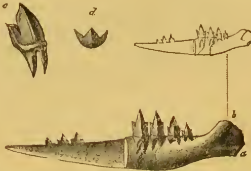
FIG. 105.—Imperfect left ramus of mandible of Spalacotherium tricuspidens (Owen), the outline figure is of the nat. size. c , d , lateral and upper views of a molar tooth. From the Middle Purbeck, Swanage, Dorset.
