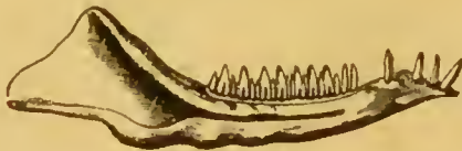
FIG. 95.—Inner view of left ramus of mandible of Dromatherium sylvestre (Emmons); from the Trias of North Carolina.
