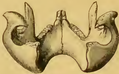
FIG. 89.—Posterior view of the lower jaw of the Wombat, Phascogomys .
