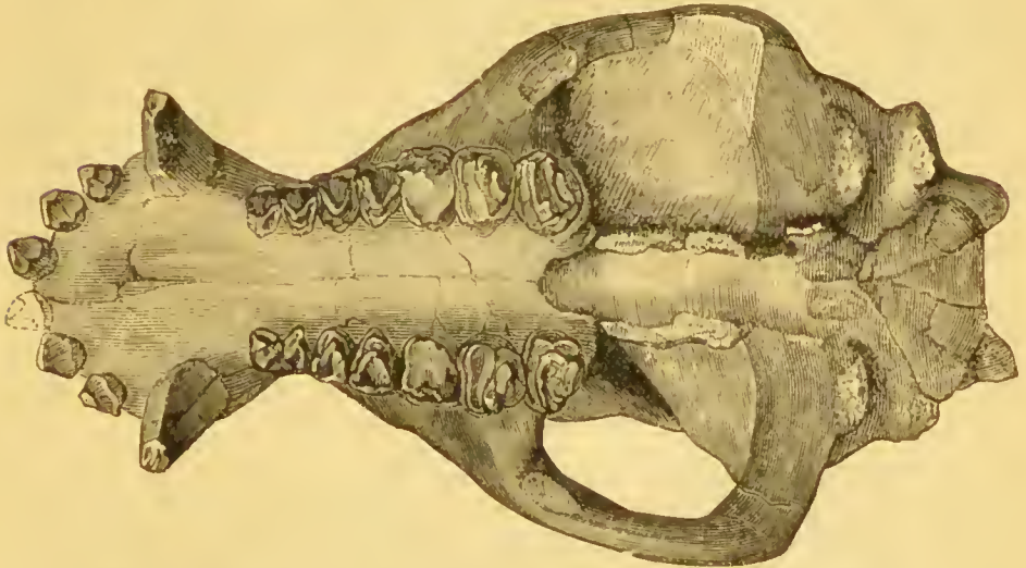
FIG. 34.—Palatal aspect of cranium of Coryphodon elephantopus (Cope) ( \frac{2}{3} nat. size), from the Wasatch Eocene, New Mexico, U.S.A. (after Cope).
