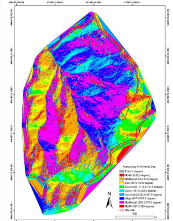
Figure 3.9. Aspect map of Kerkenes produced from GPS Data.
