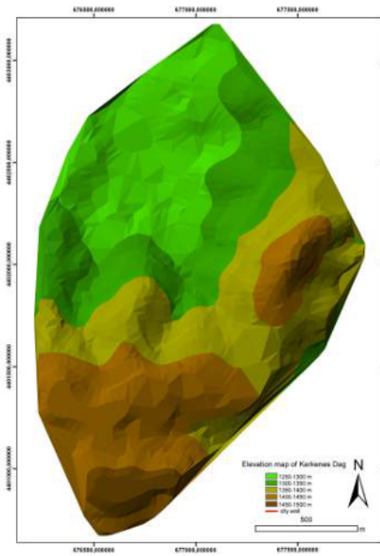
Figure 3.3. Elevation map of Kerkenes produced from extracted of six sheets of 1:25000 topographic maps as a TIN Model.
