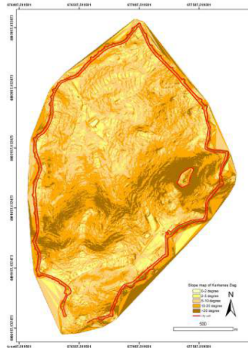
Figure 3.5. Slope map of Kerkenes produced from GPS Data.
