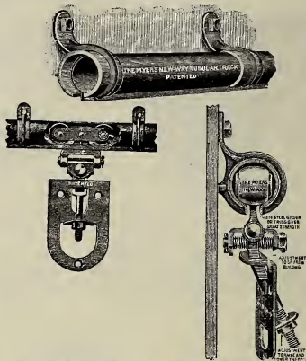
The Myers New-Way Adjustable Tandem Door Hanger For Tubular Girder Track Adjustable to and from Building and to Raise and Lower the Door
