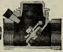
Swing Check Valve
