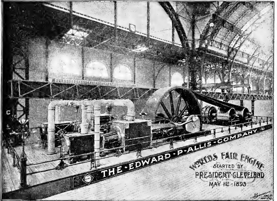
THE ALLIS ENGINE.
