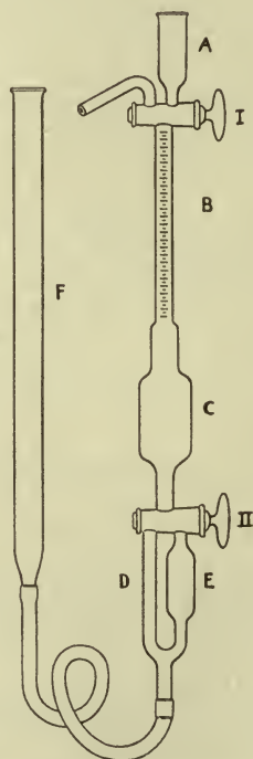
Fig. 11.—Van Slyke's apparatus for measuring the CO_2 -combining power of blood in blood plasma. For description, see context.
