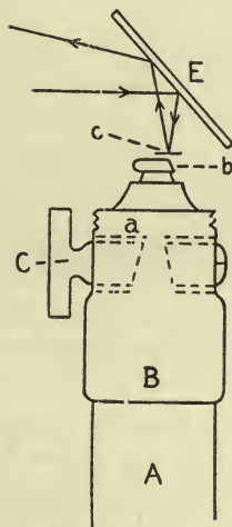
Fig. 32.—Diagram of Wiggers' optical manometer. The wide glass tube (A) (connected with the ventricle, etc.) is connected with a brass cylinder (B) provided with a stopcock (C), the lumen of which comes in apposition with a plate (a) having a small opening in it. The freedom of communication between B and a is regulated by the position of the tap. Above a is a segment capsule (b) 3 mm. in diameter and covered by rubber dam. This carries a small mirror (C) fastened so that it pivots on the chord side of the capsule. Above the capsule is arranged an inclined mirror, from which a strong beam of light is reflected on to the mirror (c) on the capsule. This beam then travels back and the mirror (E) is adjusted so that it impinges on a moving photographic plate. The slightest movements of the small mirror (C) are thus greatly magnified.
