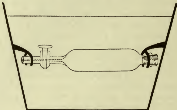
Fig. 134.—Barcroft's tonometer for determining the curve of absorption of oxygen by hemoglobin or blood. (From Starling's Physiology .)
