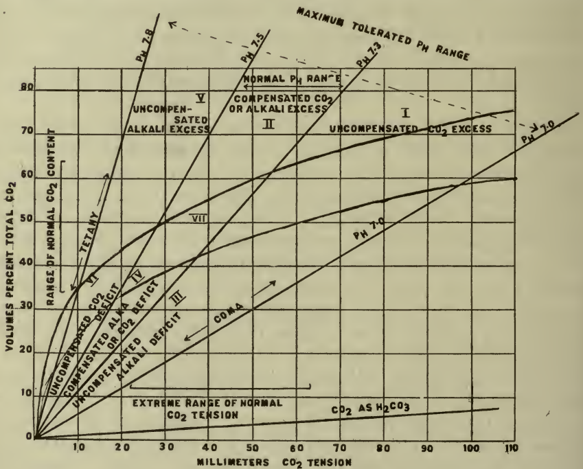
Fig. 128.—Curves showing relationship between total CO_2 in solution and P_H at varying CO_2 pressure. (Redrawn from D. D. Van Slyke.)
