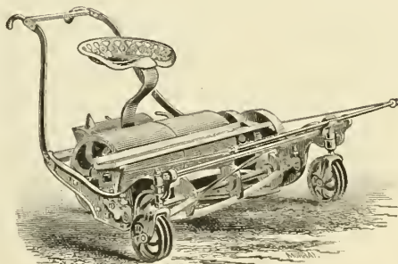
New Excelsior Horse Lawn Mower.
