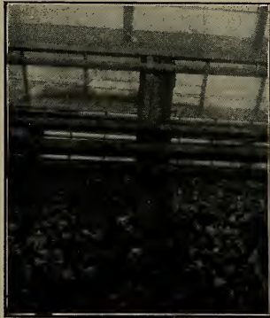
15.—Fastening pipes to posts by bent wire nails.
