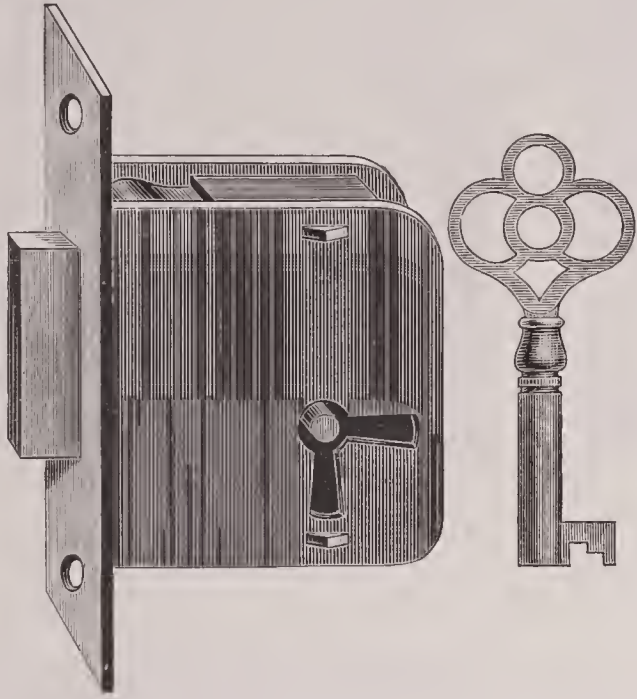
No. 312. 2 3/4 inch, $2.25. Iron. Brass Selvedge, Broad Heavy Bolt, Tumbler. 1 inch from Selvedge to Key Pin.
