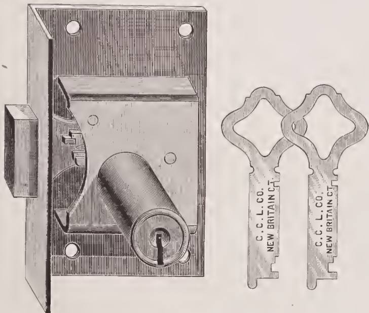
No. 331. 2 1/2 inch, $5.00. Iron. Not Polished, Heavy Bolt, 2 Secure Levers, 2 Nickel-Plated Flat Steel Keys to each Lock, all different, made for 7/8 inch wood. 3/4 inch from Selvedge to center of Cylinder.
