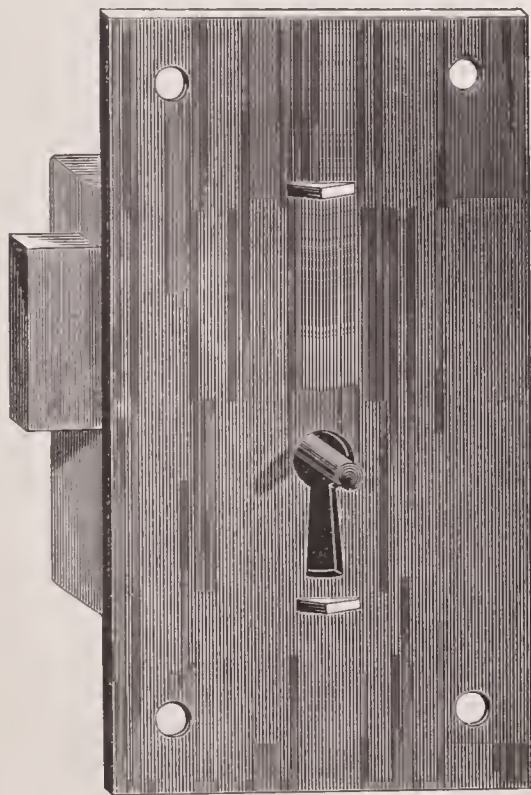
No. 712. 3½ x 2 inch, $2.25. Iron. Solid Square Box, Broad Heavy Bolt, shoots right and left, 2 Secure Levers, Fancy Bow Keys, all different.
