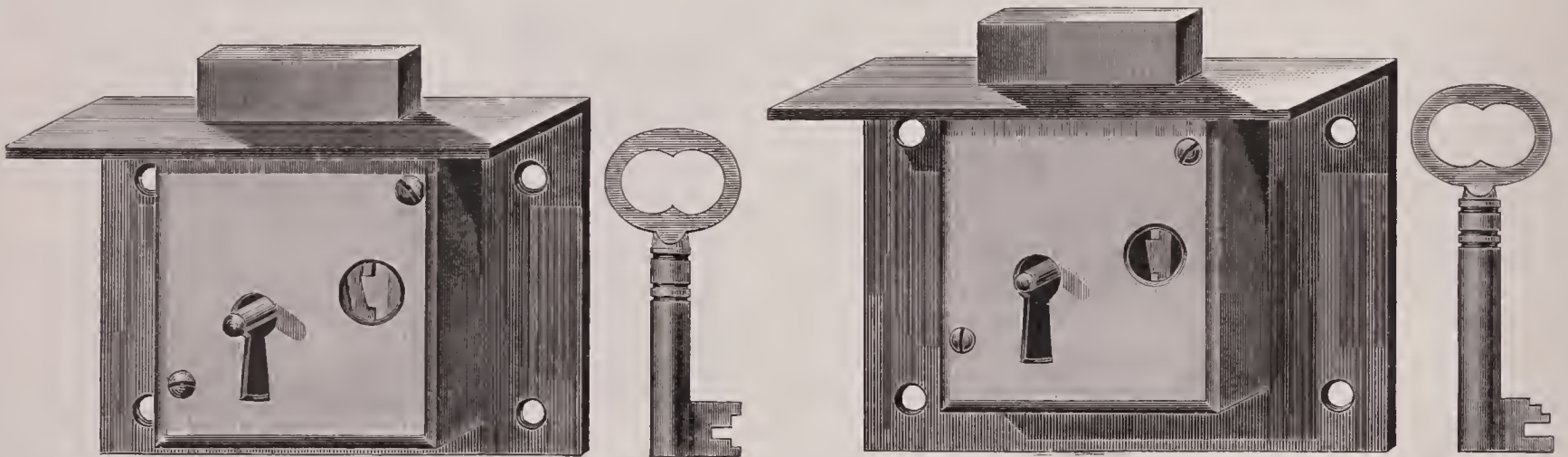
No. 0477. 2½ inch, $7.50. Brass. Square Selvedge, Solid Square Brass Box, Screwed, Broad Heavy Bolt, 1 Secure Lever, 3 Wards, Fine Flat Bow Keys, all different. ⅞ inch from Selvedge to Key Pin.
