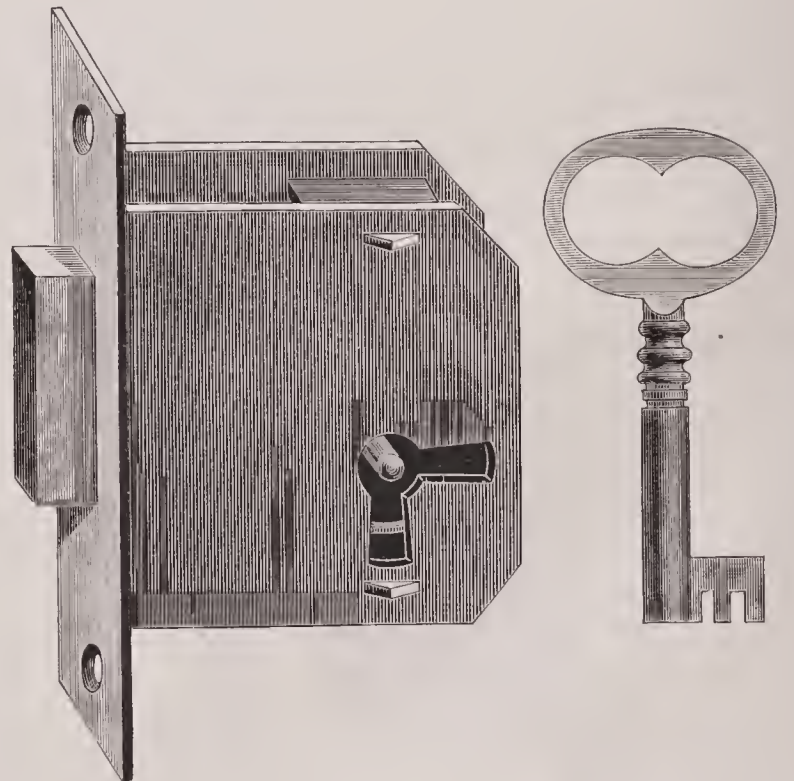
No. 317. 3 inch, $3.25. Iron. Brass Selvedge, Broad Heavy Bolt, 1 Ward, Tumbler. 1 1/4 inch from Selvedge to Key Pin.
