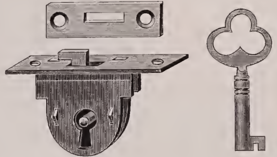
No. 18. 1½ inch, $1.00. Mortise, Brass Selvedge, Bolt and Strike. ⅜ inch from Selvedge to Key Pin.
