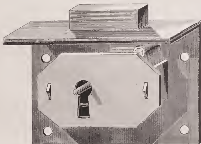
No. 421, P. 2\frac{3}{4} inch, $1.50. Iron. Square Brass Sledge. Broad Heavy Bolt, Tumbler, 1 Ward. 1\frac{1}{8} inch from Sledge to middle of Key-hole.
