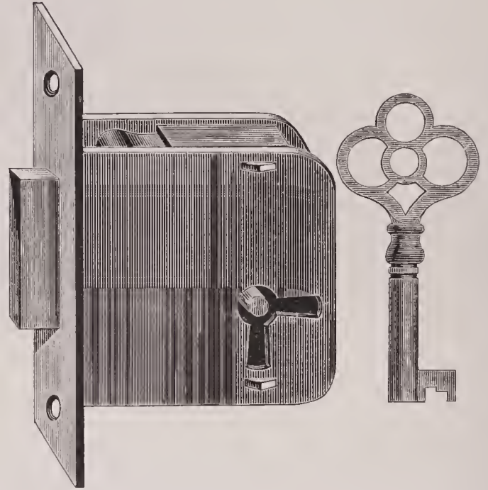
No. 313. 2 3/4 inch, $2.25. Iron. Brass Selvedge, Broad Heavy Bolt, Tumbler. 1 1/8 inch from Selvedge to Key Pin.
