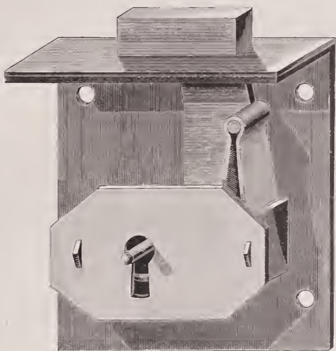
No. 421, L. 2\frac{3}{4} inch, $1.70. Iron. Square Brass Sledge. Broad Heavy Bolt, Tumbler, 1 Ward. 2 inches from Sledge to middle of Key-hole.
