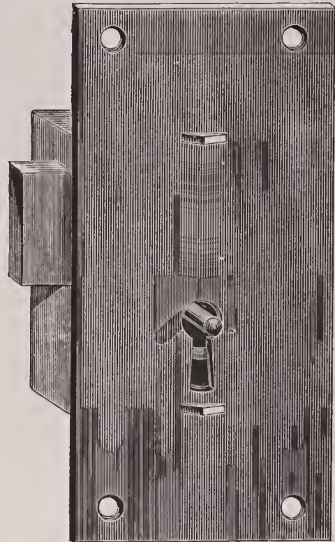
No. 710. 3\frac{1}{2} x 1\frac{1}{4} inch, $1.75. Iron. Solid Square Box, Broad Bolt, shoots right and left, Tumbler.
