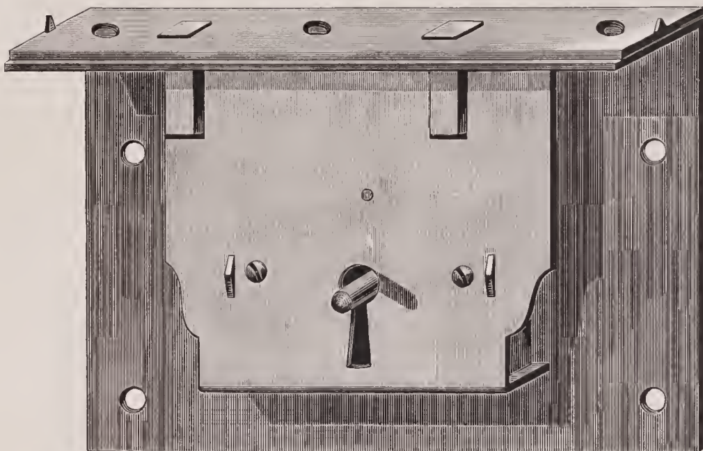
No. 72. 4 inch, $5.00. Iron. Screwed, 2 Secure Levers, Fine Flat Bow Keys, all different. 1\frac{1}{2} inch from Selvedge to Key Pin.
