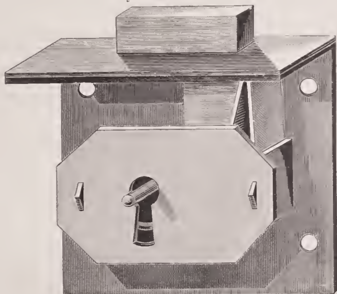
No. 421, N. 2\frac{3}{4} inch, $1.50. Iron. Square Brass Sledge. Broad Heavy Bolt, Tumbler, 1 Ward. 1\frac{1}{2} inch from Sledge to middle of Key-hole.
