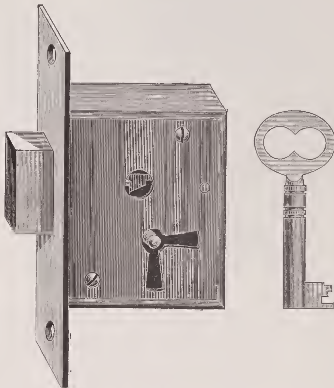
No. 316. 3 inch, $4.25. Iron. Brass Selvedge, Solid Square Box, Screwed, Heavy Bolt, 2 Secure Levers, Fine Flat Bow Keys, all different. 3/8 inch from Selvedge to Key Pin.
