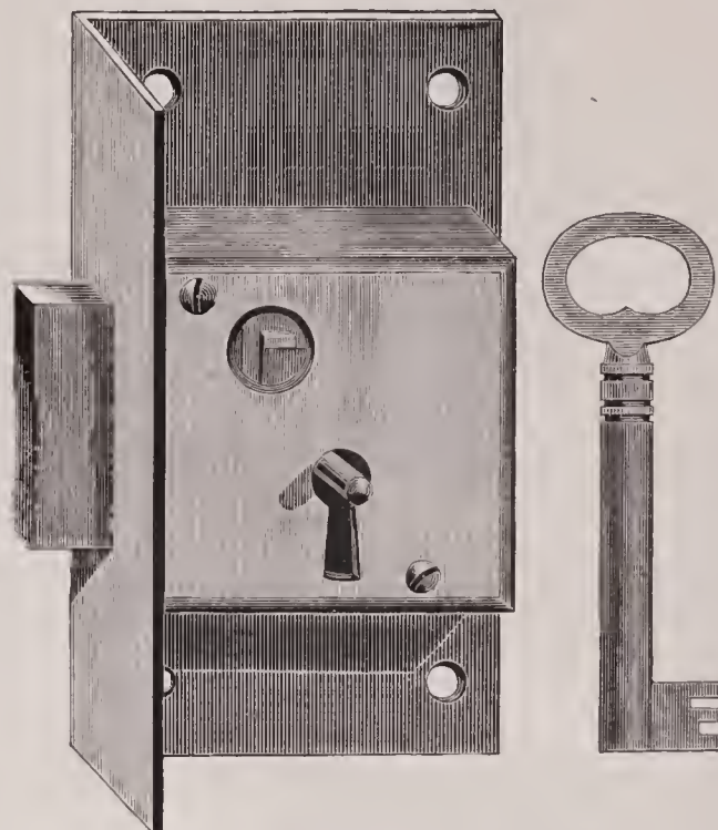
No. 0266. 3 inch, $8.50. Brass. Square Selvedge, Solid Square Brass Box, Screwed, Broad Heavy Bolt, 1 Secure Lever, 3 Wards, Fine Flat Bow Keys, all different. \frac{7}{8} inch from Selvedge to Key Pin.
