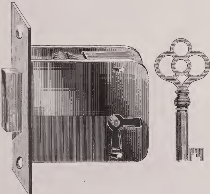
No. 314. 2 3/4 inch, $2.75. Iron. Brass Selvedge, Broad Heavy Bolt, Tumbler. 1 3/8 inch from Selvedge to Key Pin.
