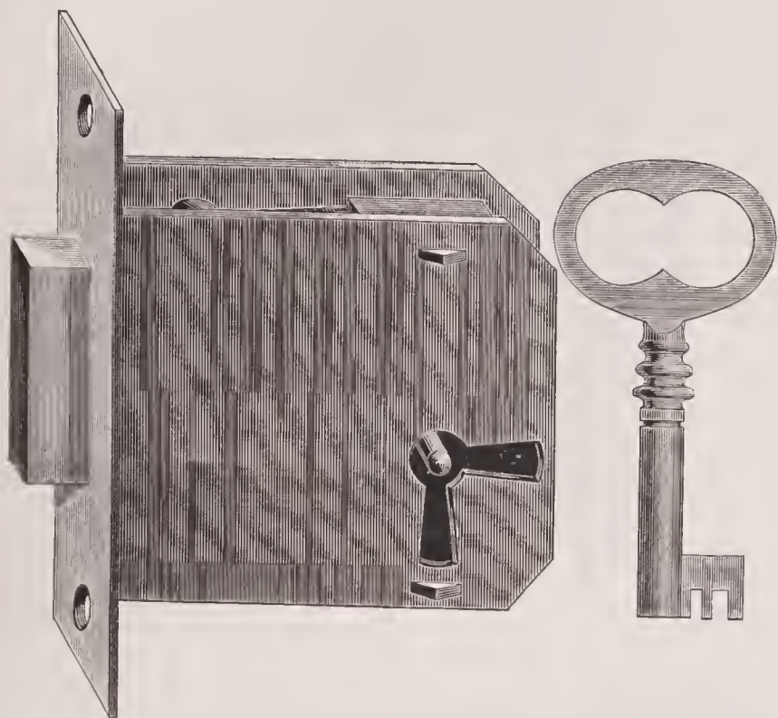
No. 318. 3 inch, $3.38. Iron. Brass Selvedge, Broad Heavy Bolt, 1 Ward, Tumbler. 1 3/4 inch from Selvedge to Key Pin.
