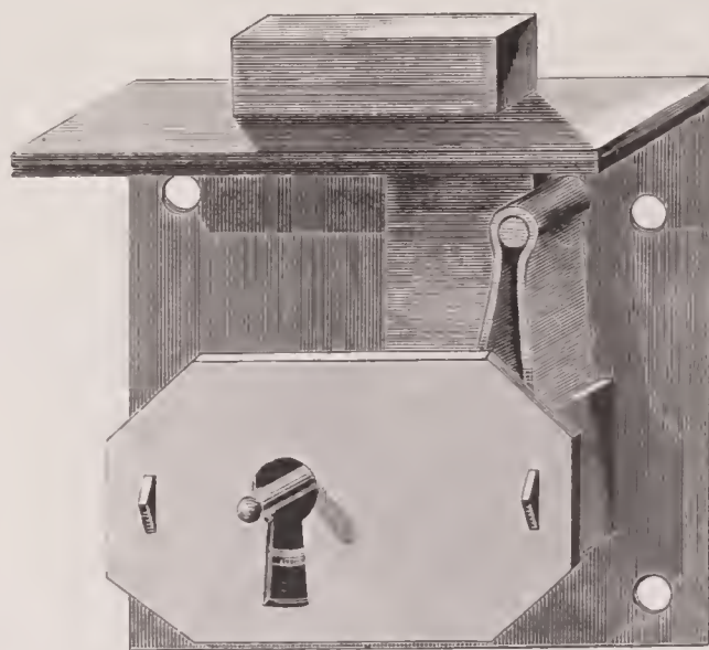
No. 421, M. 2\frac{3}{4} inch, $1.60. Iron. Square Brass Sledge. Broad Heavy Bolt, Tumbler, 1 Ward. 1\frac{3}{4} inch from Sledge to middle of Key-hole.
