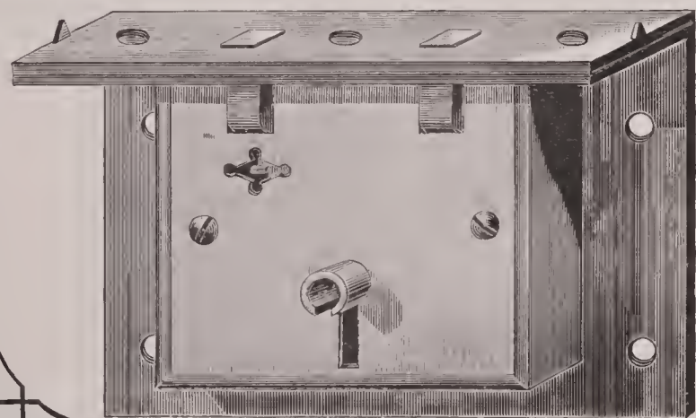
No. O125. 2 1/2 inch, $9.50. Brass. Same as No. 124. 3 Secure Levers.
