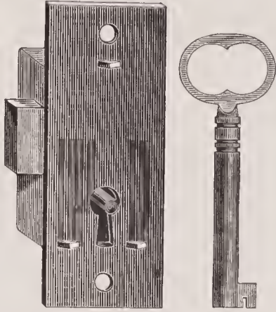
No. 700. 1\frac{1}{2} \times \frac{3}{4} inch, $1.50. Iron. Solid Square Box, Bolt shoots right and left, Tumbler, Fine Flat Bow Keys.
