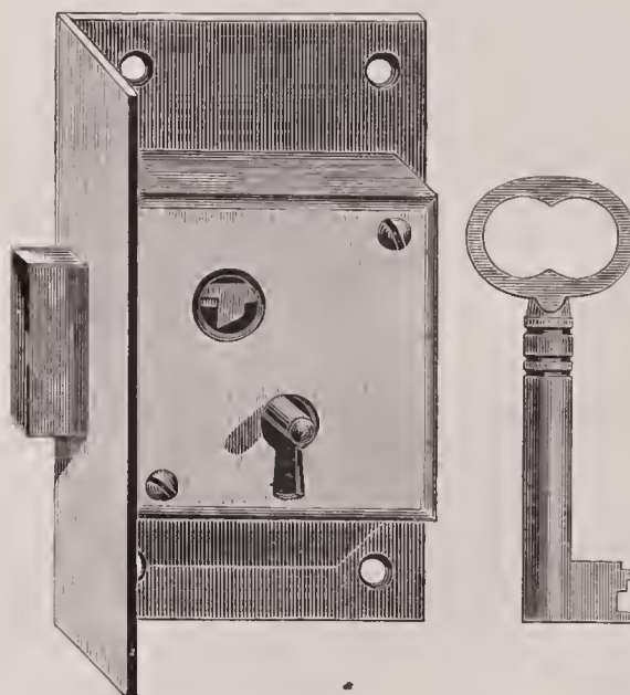
No. 0270. 2½ inch, $2.75. Brass. Square Selvedge, Solid Square Box, Screwed, Heavy Bolt, 1 Secure Lever, Fine Flat Bow Keys, Assorted, 6 changes in each dozen. \frac{3}{4} inch from Selvedge to Key Pin.
