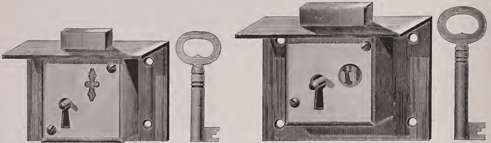
No. 0475. 2½ inch, $4.75. Brass. Square Selvedge, Solid Square Brass Box, Screwed, Broad Heavy Brass Bolt, 2 Secure Levers, Fine Flat Bow Brass Keys, all different. ⅝ inch from Selvedge to Key Pin.
