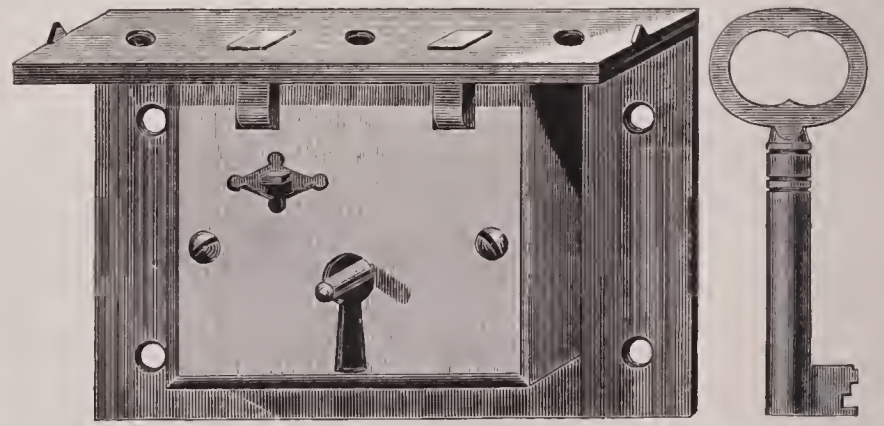
No. 105. 2 3/4 inch, $3.75. Iron. Square Selvedge, Screwed, Solid Box, 2 Secure Levers, Fine Flat Bow Keys, all different. 1 inch from Selvedge to Key Pin.
