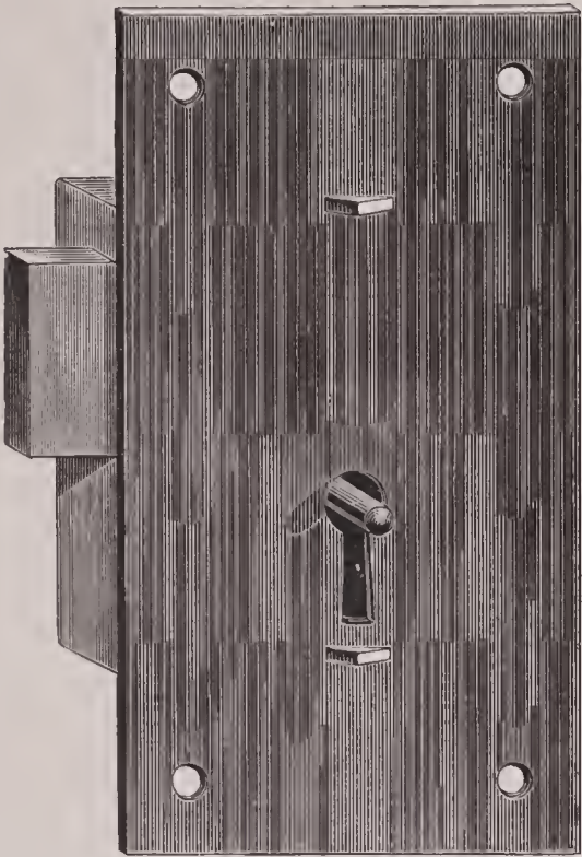
No. 709. 3\frac{1}{2} x 2 inch, $1.87. Iron. Solid Square Box, Broad Bolt, shoots right and left, Tumbler.
