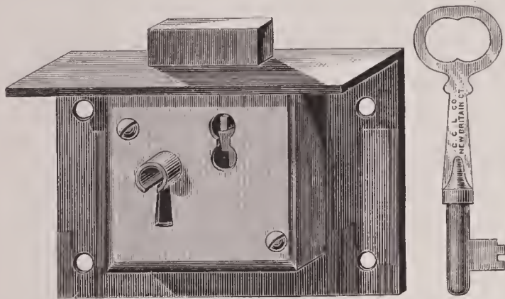
No. 572. 2¼ inch, $4.25. Iron. Square Selvedge, Solid Square Box, Screwed, Broad Heavy Bolt, 2 Secure Levers, Solid Nickel Bit Keys, all different. ⅝ inch from Selvedge to center of Tube.
