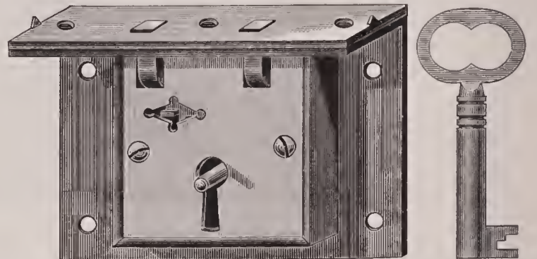
No. 103. 2 1/4 inch, $3.37. Iron. Square Selvedge, Screwed, Solid Box, 2 Secure Levers, Fine Flat Bow Keys, all different. 7/8 inch from Selvedge to Key Pin.
