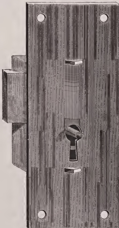
No. 711. 3\frac{1}{2} x 1\frac{1}{2} inch, $2.00. Iron. Solid Square Box, Broad Bolt, shoots right and left, Tumbler.
