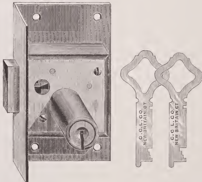
No. 334. 2 1/2 inch, $6.00. Iron. Square Selvedge, Solid Square Box, Screwed, Heavy Bolt, 2 Secure Levers, 2 Nickel-Plated Flat Steel Keys to each Lock, all different, made for 7/8 inch wood. 3/4 inch from Selvedge to center of Cylinder.
