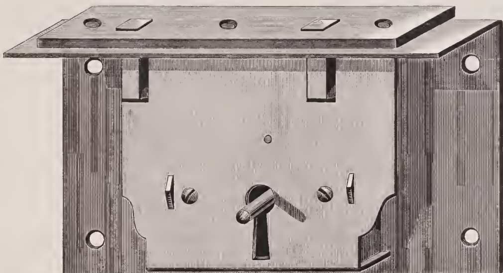
No. 73. 4 inch, $4.50. Iron. Screwed, 2 Secure Levers, Flat Bow Keys, all different. 1\frac{1}{2} inch from Selvedge to Key Pin.
