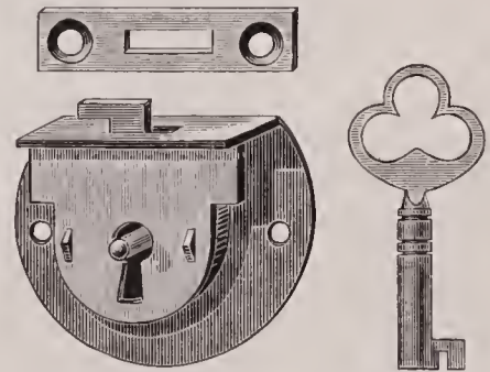
No. 20. 1 inch, $1.00. Iron. Brass Bolt and Strike. ⅜ inch from Selvedge to Key Pin.
