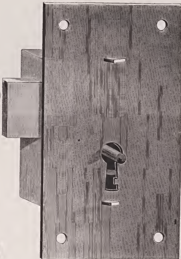
No. 715. 4 x 2¼ inch, $3.00. Iron. Solid Square Box, Broad Heavy Bolt, shoots right and left, Tumbler, 1 Ward.
