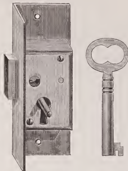
No. 0261. 2½ inch, $5.00. Brass. Square Selvedge, Screwed, Solid Box, 1 Secure Lever, assorted, Fine Flat Bow Keys. \frac{3}{8} inch from Selvedge to Key Pin.
