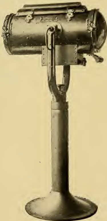
Fig. 22.—Marine Searchlight on High Stand.
