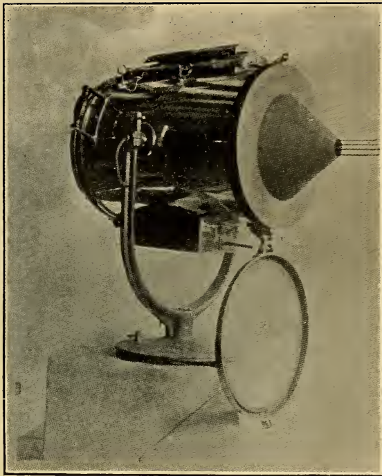
Fig. 23.—Marine Searchlight, with Funnel-shaped Attachment.
